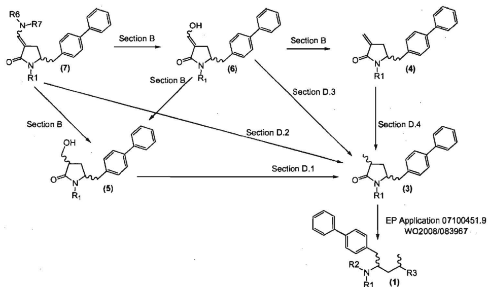
Scheme 5
