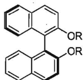
(S)-BINOL
