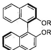
(R)-BINOL
