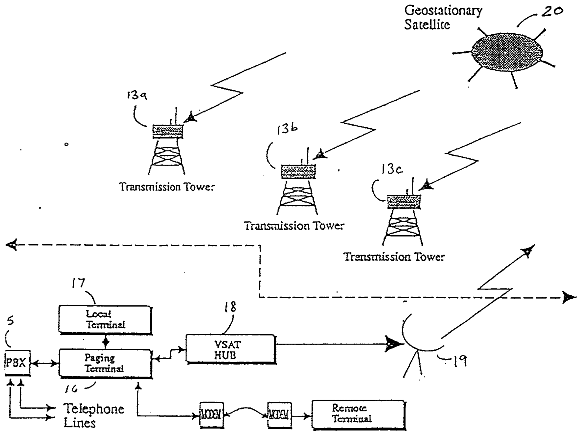
Paging Central Office Prior Art FIG. 2
