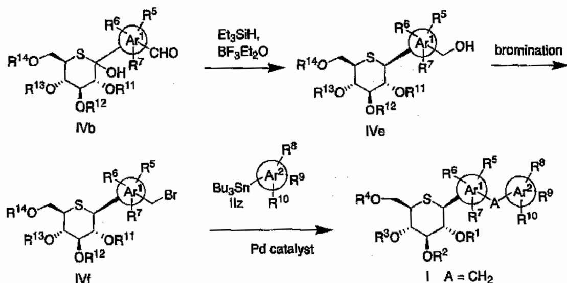
Scheme 13
