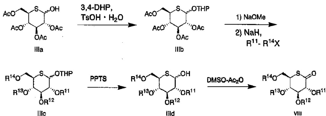
[0168] Scheme 9
