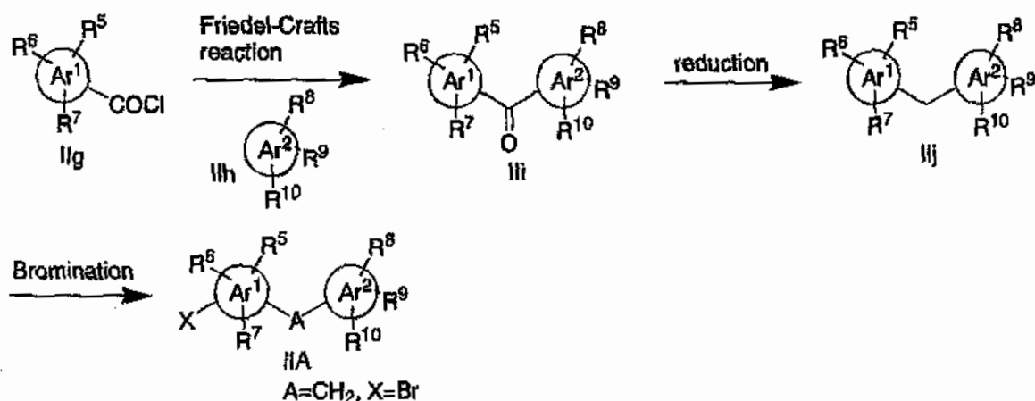
Scheme 7
