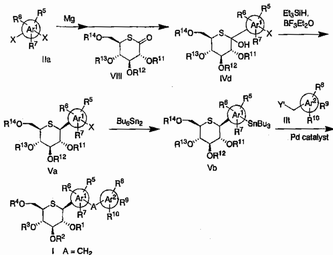
Scheme 12
