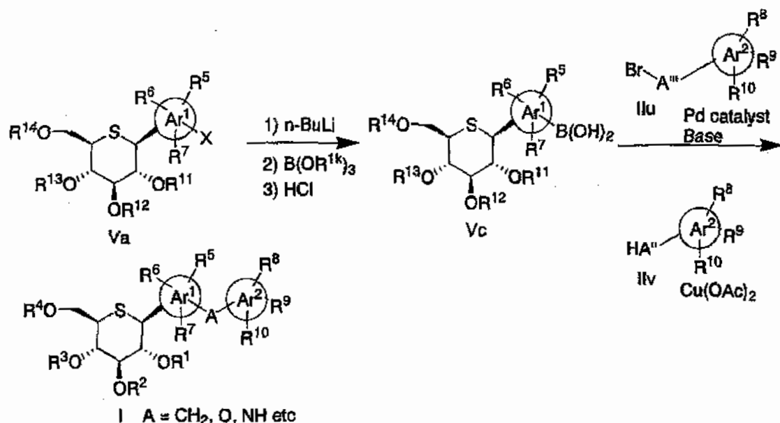
Scheme 14
