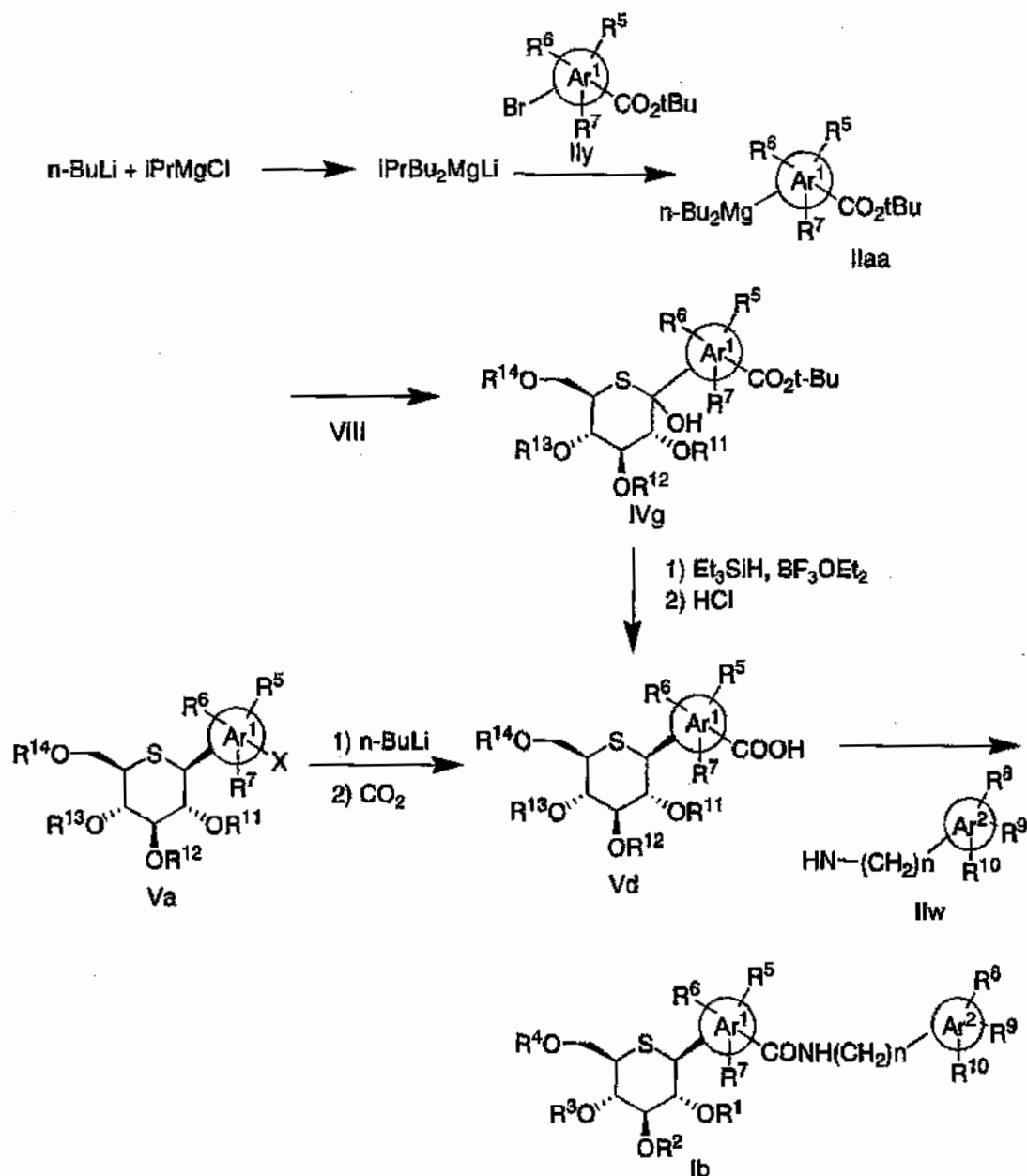
Scheme 15
