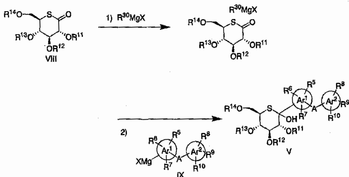
Scheme 3
