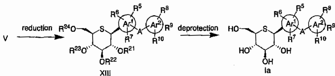
Scheme 4
