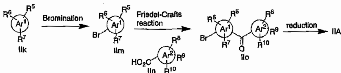
Scheme 8
