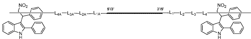
Formula (I''-b)
