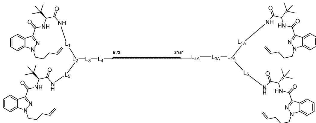
Formula (IV''-b-1)
