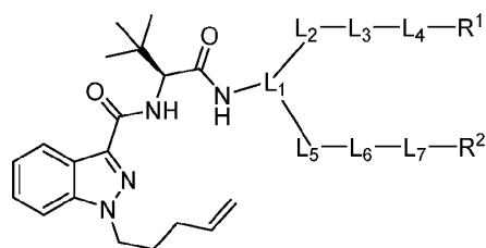
Formula (VII-a)
