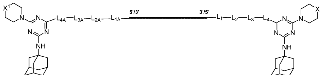
Formula (I''-a-1)
