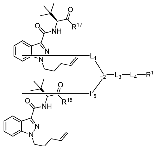
Formula (V)
