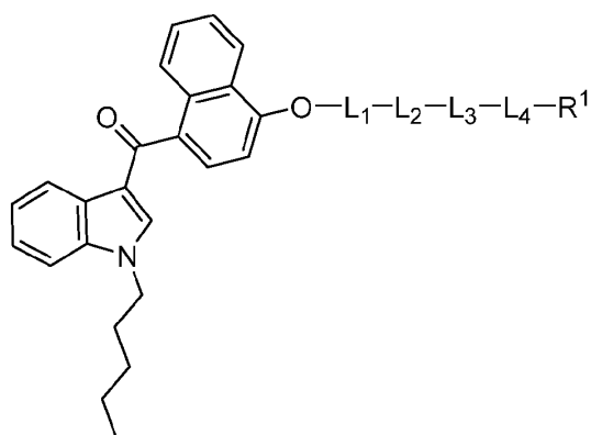
Formula (VIII-a-2)
