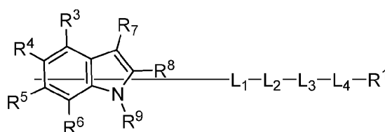
Formula (VIII)
