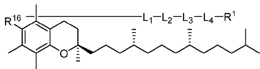
Formula (X)
