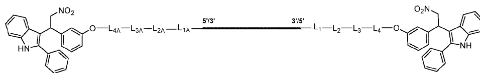
Formula (I''-b-2)
