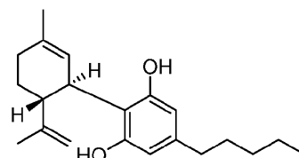
Cannabidiol
