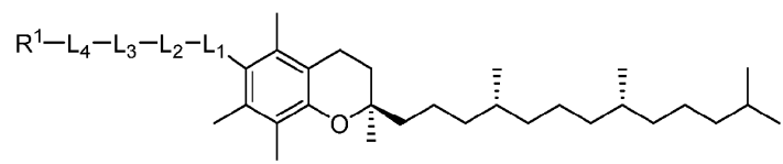
Formula (X-a)
