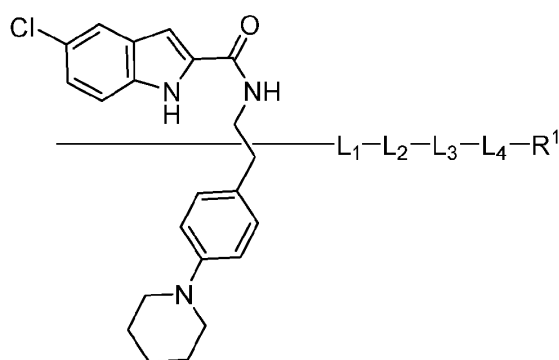
Formula (VIII-b)
