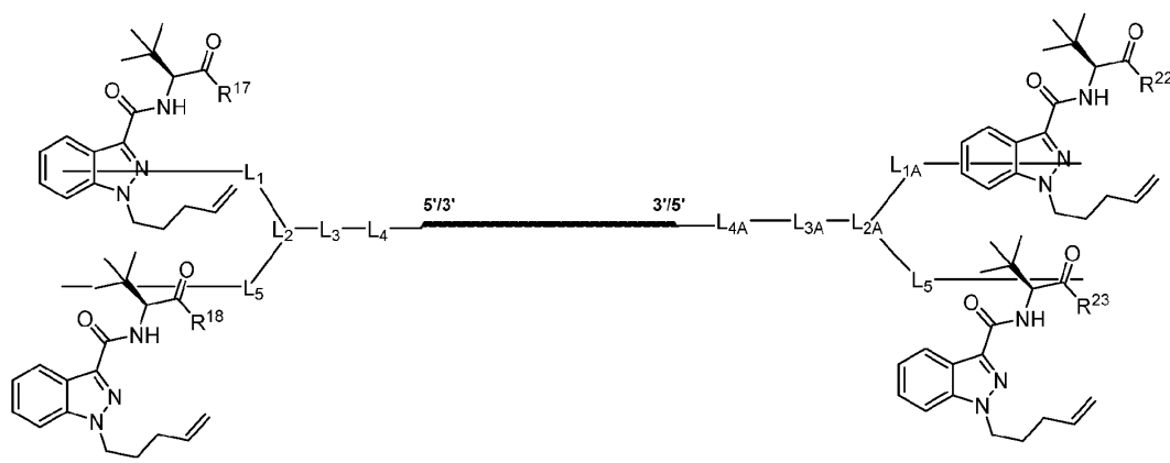
Formula (IV''-a)
