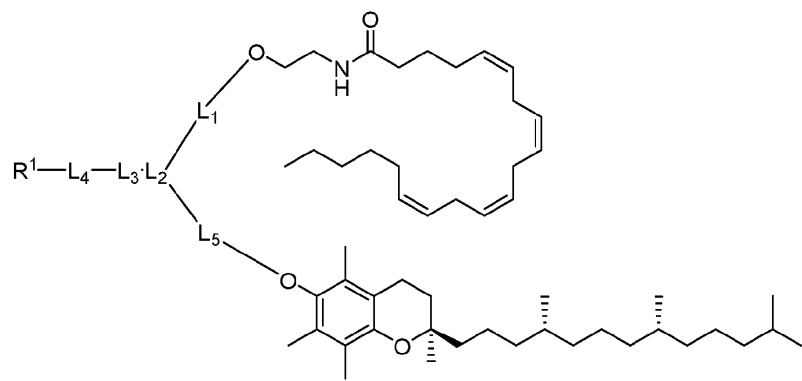
Formula (IX-a)
