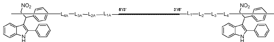
Formula (I''-b)
