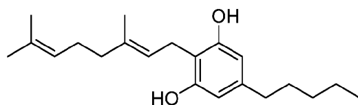
Cannabigerol
