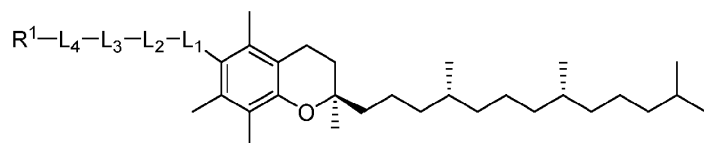
Formula (X-a)
