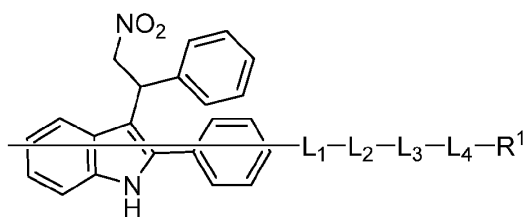
Formula (VIII-c)
