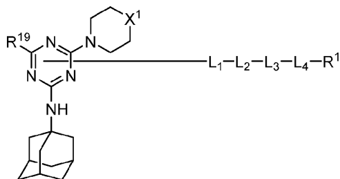
Formula (IX)
