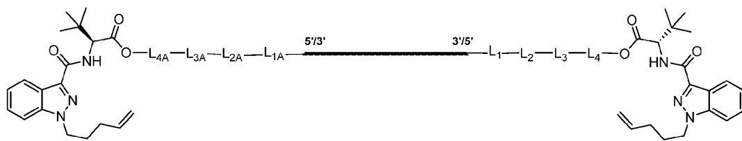
Formula (XII-c)
