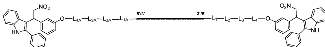
Formula (I''-b-2)
