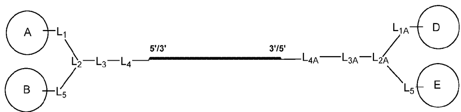
Formula (IV'')
