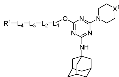
Formula (IX-a-2)
