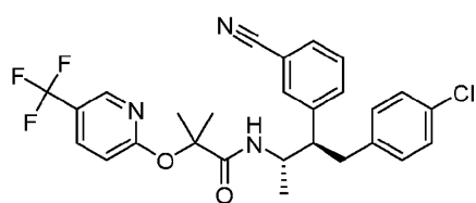
Taranabant
