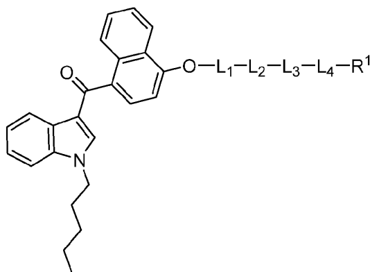
Formula (VIII-a-2)
