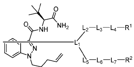
Formula (VII)
