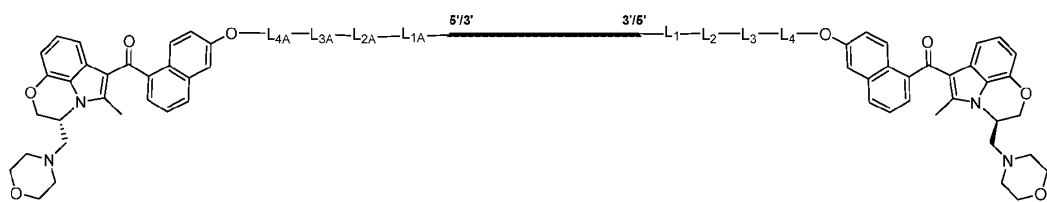
Formula (I''-c-2)
