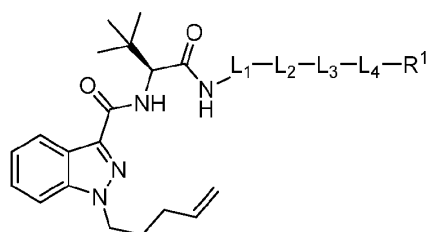
Formula (II-a)
