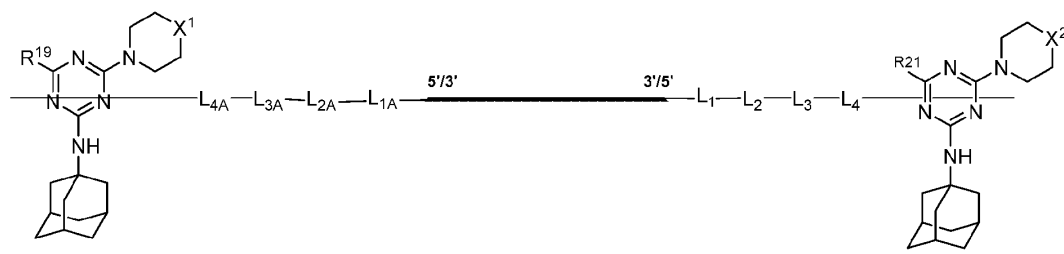
Formula (I''-a)
