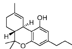
Tetrahydrocannabivarin
