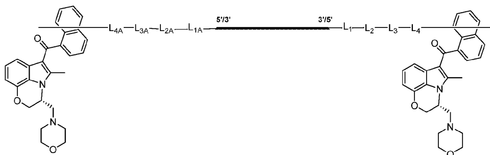
Formula (I''-c).
