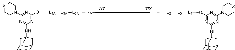
Formula (I''-a-2)
