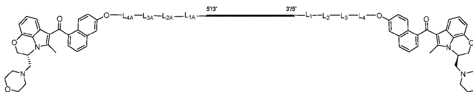
Formula (I''-c-2)
