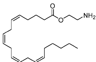
Virodhamine
