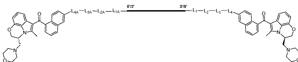
Formula (I''-c-1)
