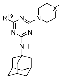
Formula (IX)
