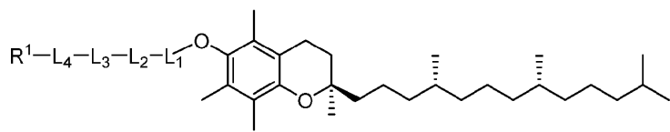
Formula (X-a-1)
