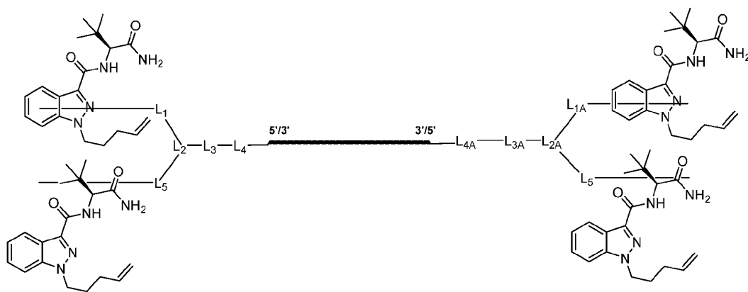
Formula (IV''-b)
