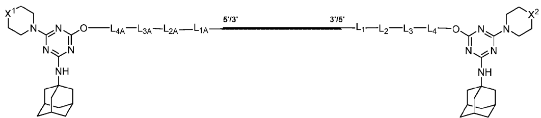
Formula (I''-a-2)
