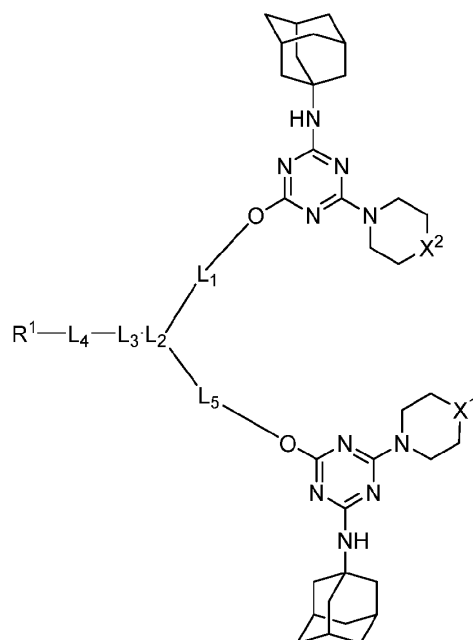
Formula (XI-a)
