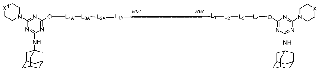
Formula (I''-a-2)
