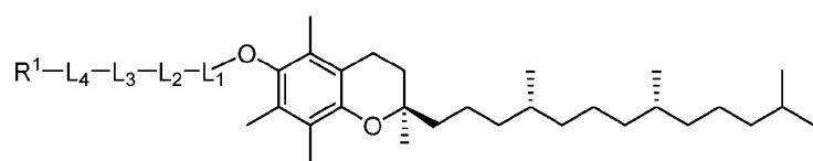
Formula (X-a-1)
