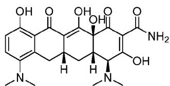
Minocycline
