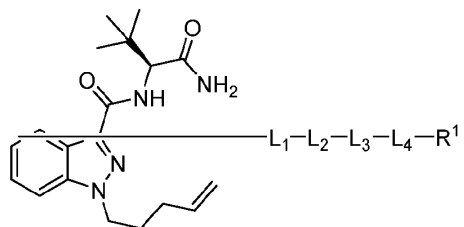
Formula (II)
