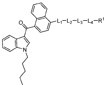
Formula (VIII-a-1)
