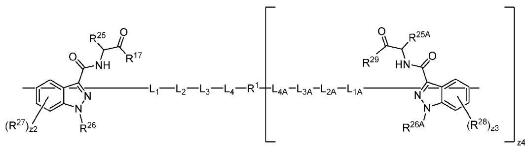
Formula (XII)
