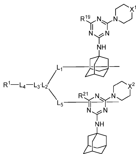
Formula (XI)
