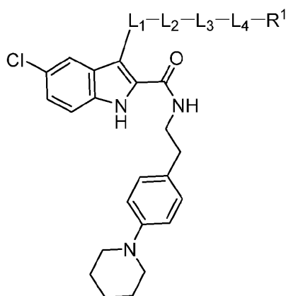
Formula (VIII-b-1)
