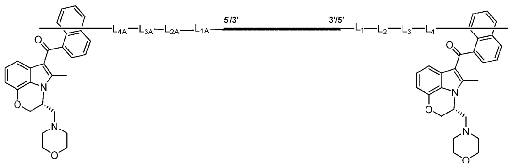
Formula (I''-c).
