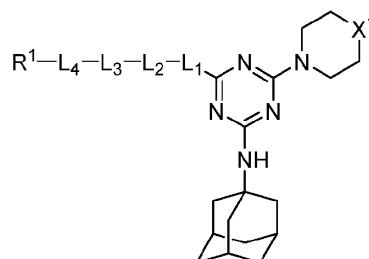
Formula (IX-a-1)
