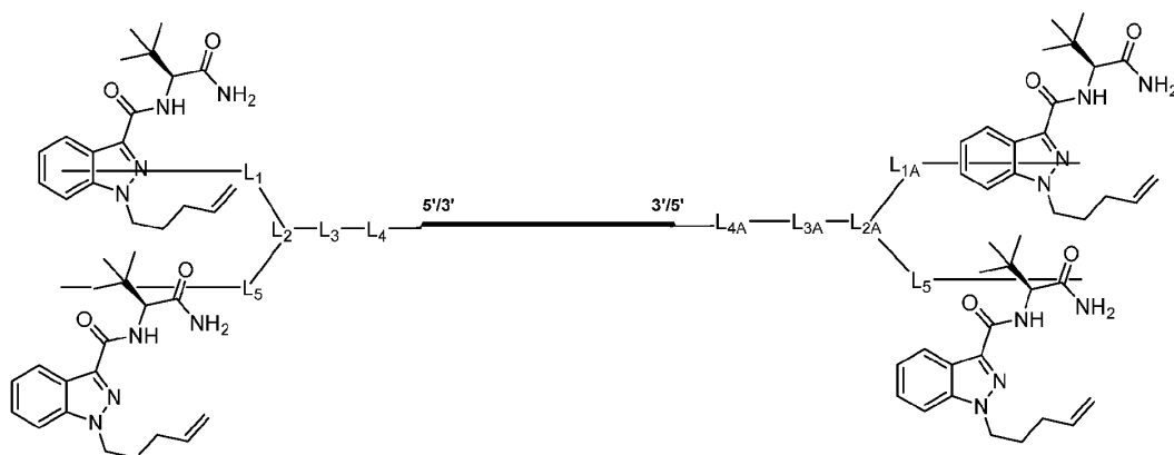
Formula (IV''-b)
