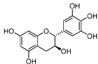
Epigallocatechin
