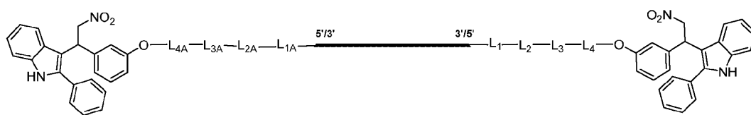
Formula (I''-b-2)
