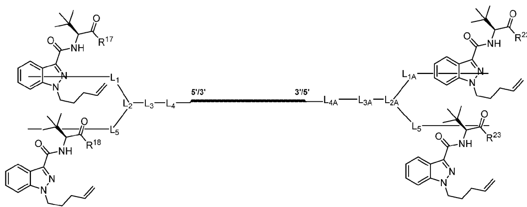
Formula (IV''-a)
