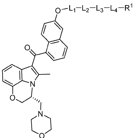
Formula (VIII-d-2)
