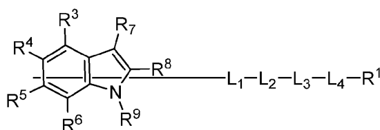
Formula (VIII),
