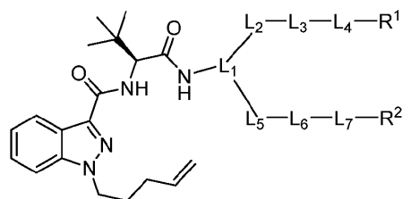
Formula (VII-a)
