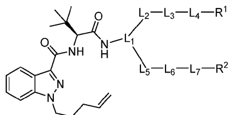
Formula (VII-a)
