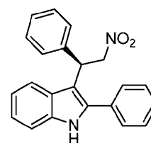
GAT228
