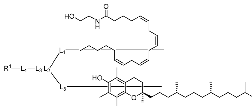
Formula (IX)
