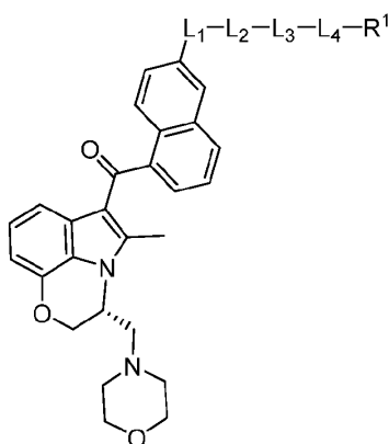
Formula (VIII-d-1)
