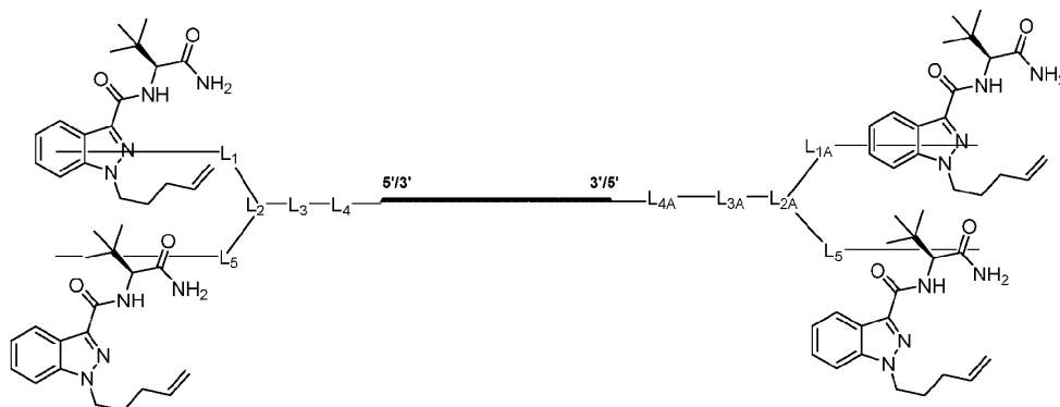
Formula (IV''-b)
