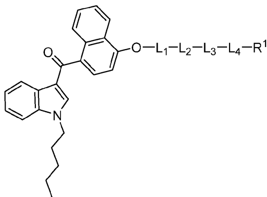
Formula (VIII-a-2)
