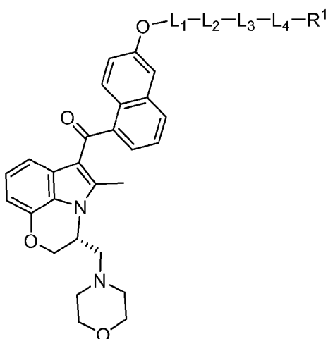
Formula (VIII-d-2)
