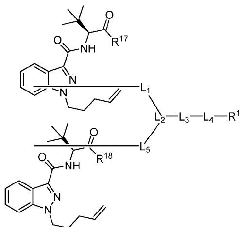
Formula (V)
