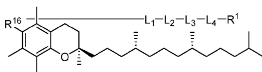
Formula (X)
