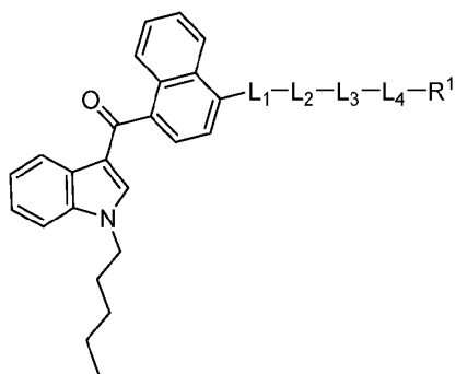
Formula (VIII-a-1)
