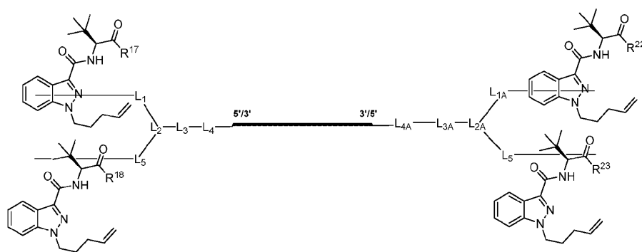
Formula (IV''-a)
