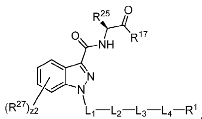
Formula (XII-a-1)
