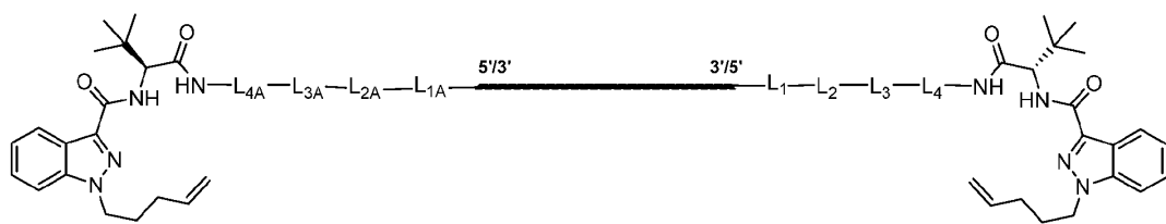
Formula (XII-b)
