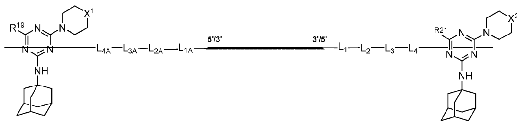
Formula (I''-a)
