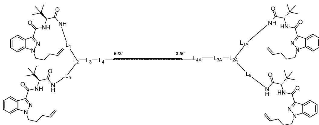
Formula (IV''-b-1)
