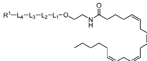
Formula (III-a)
