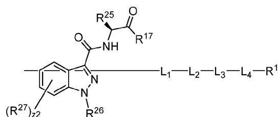
Formula (XII-a)
