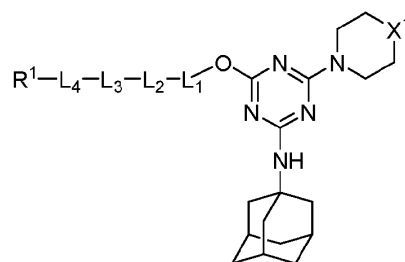
Formula (IX-a-2)
