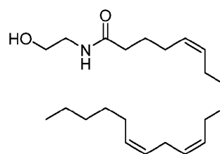
Anandamide
