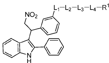
Formula (VIII-c-1)
