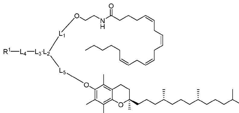
Formula (IX-a)
