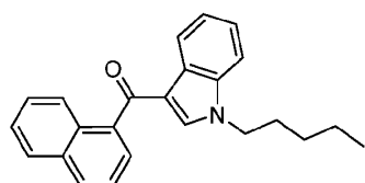
JWH-018
