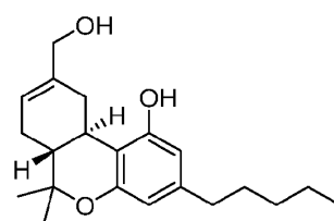
11-hydroxy-THC
