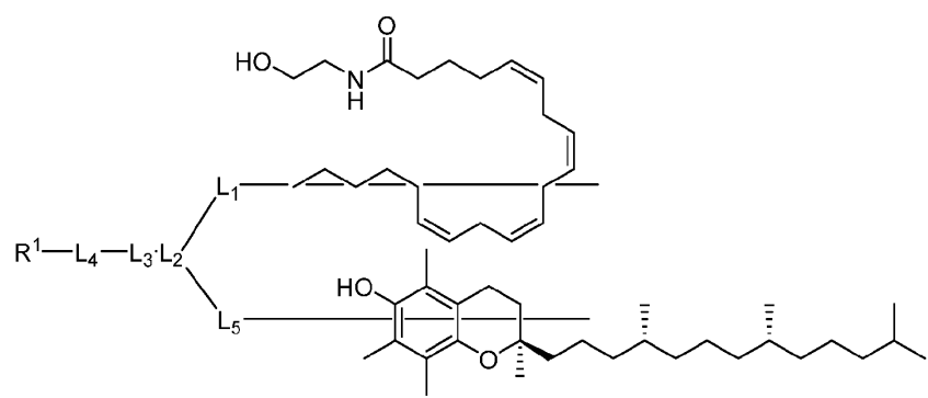
Formula (IX)
