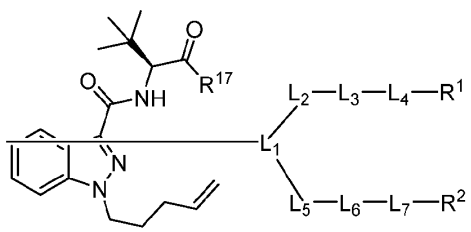
Formula (VII)
