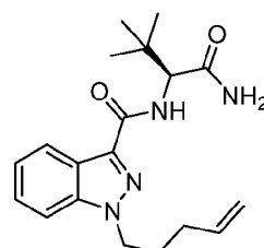
(S)-N-(1-amino-3,3-dimethyl-1-oxobutan-2-yl)-1-(pent-4-en-1-yl)-1H-indazole-3-carboxamide
