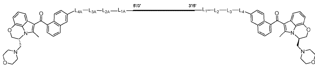
Formula (I''-c-1)
