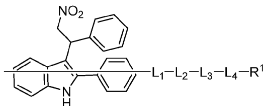
Formula (VIII-c)
