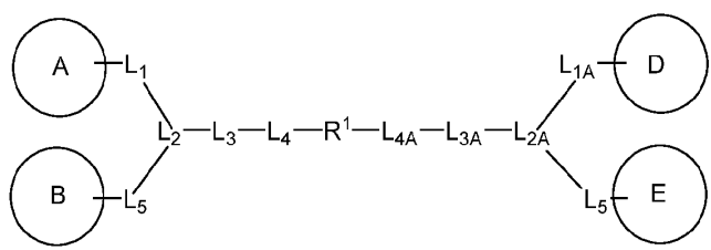
Formula (IV')
