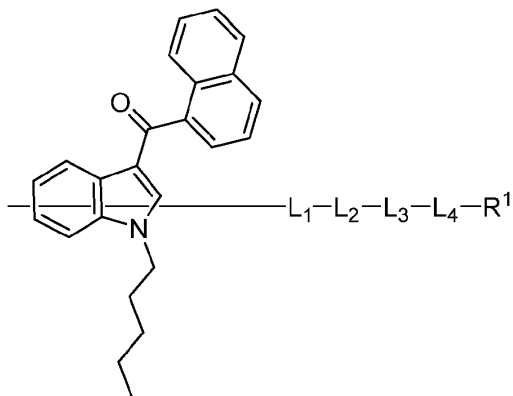
Formula (VIII-a)
