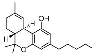
Tetrahydrocannabinol
