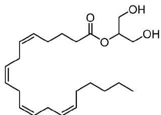
2-arachidonoylglycerol
