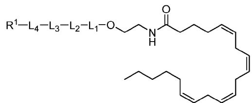
Formula (III-a)
