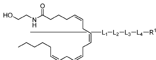
Formula (III)
