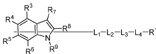
Formula (VIII)
