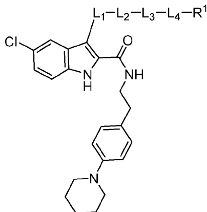
Formula (VIII-b-1)
