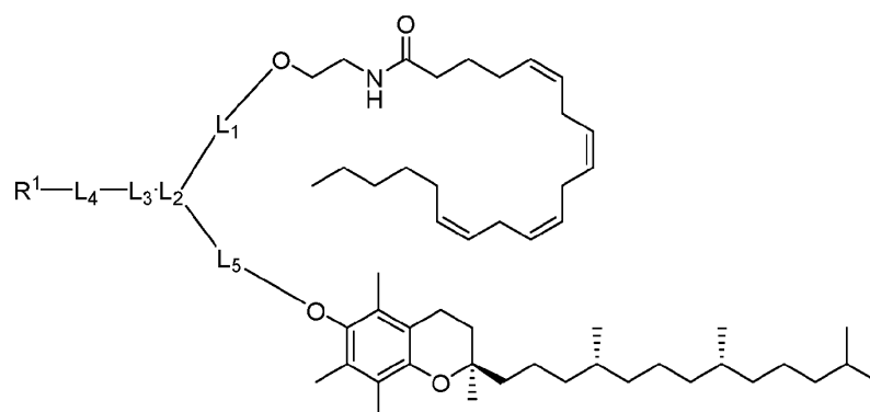
Formula (IX-a)
