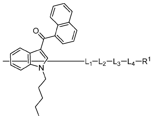
Formula (VIII-a)
