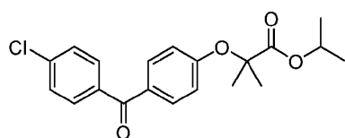
Fenofibrate
