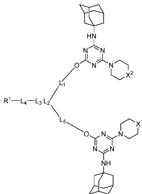
Formula (XI-a)
