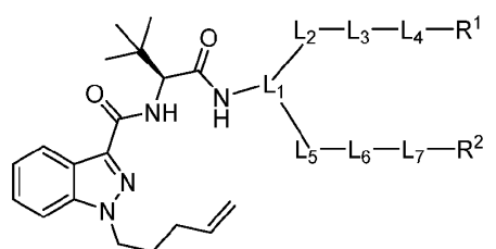
Formula (VII-a)
