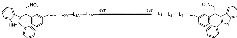
Formula (I''-b-1)
