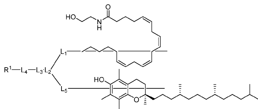
Formula (IX)
