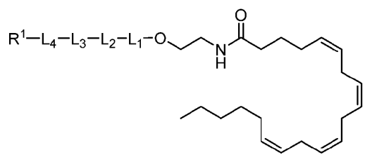
Formula (III-a)
