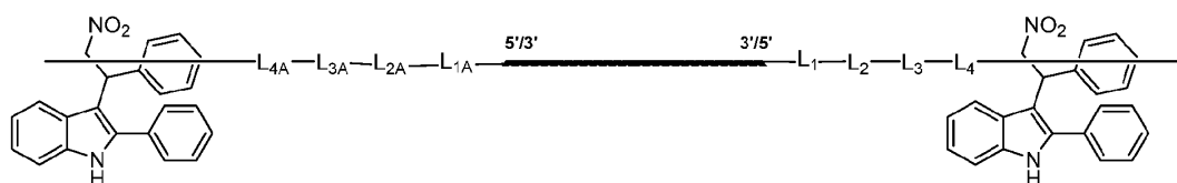
Formula (I''-b)
