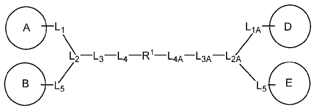
Formula (IV')
