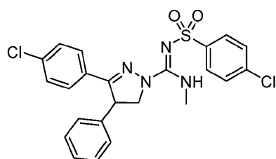
Ibipinabant
