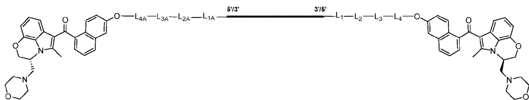
Formula (I''-c-2)
