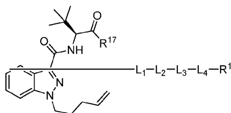
Formula (II)
