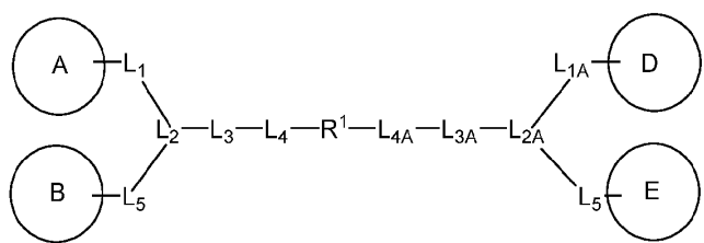
Formula (IV')
