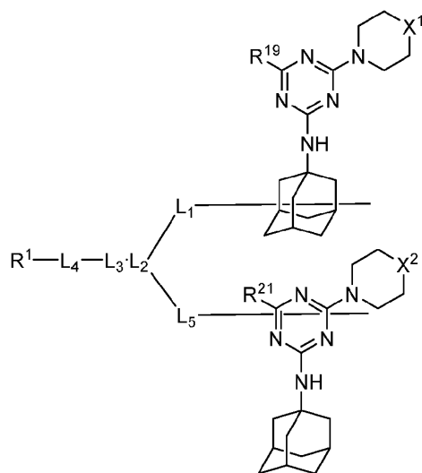
Formula (XI)
