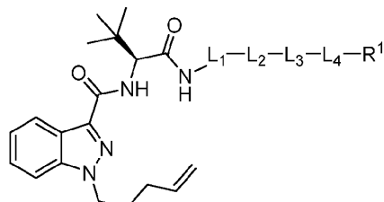
Formula (II-a)
