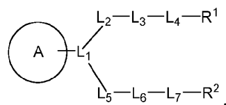
Formula (VI)
