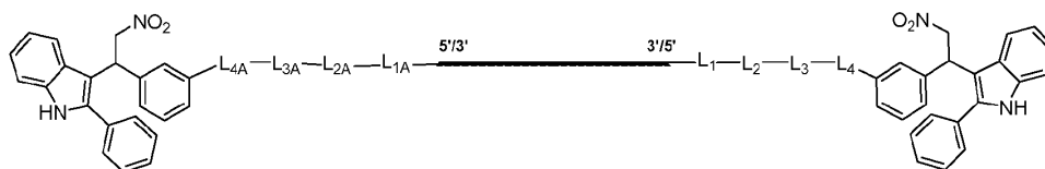
Formula (I''-b-1)
