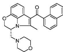
WIN 55,212-2
