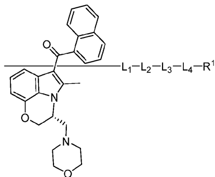
Formula (VIII-d)
