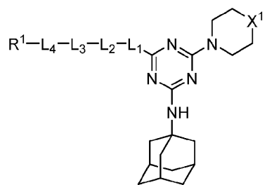
Formula (IX-a-1)
