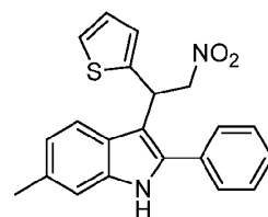
ZCZ-011
