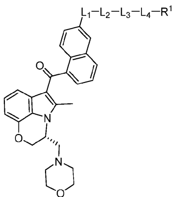
Formula (VIII-d-1)
