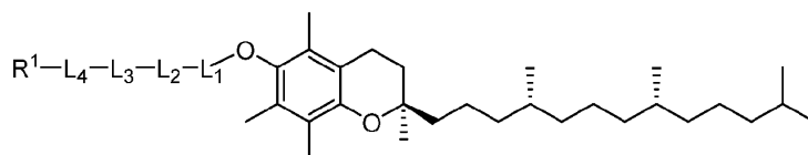
Formula (X-a-1)
