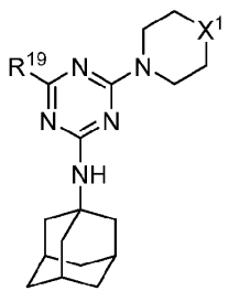
Formula (IX)
