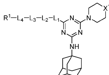
Formula (IX-a-1)
