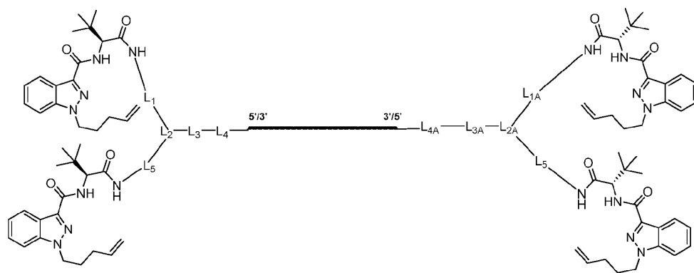
Formula (IV''-b-1)
