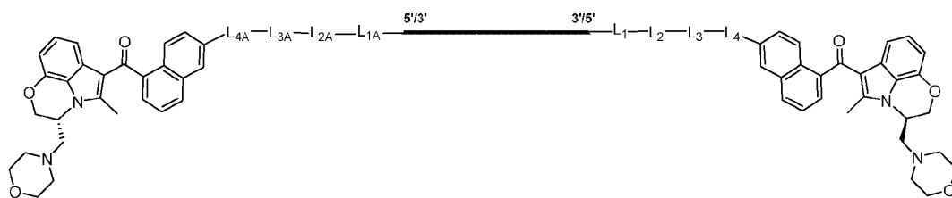
Formula (I''-c-1)
