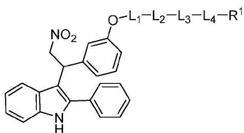
Formula (VIII-c-2)
