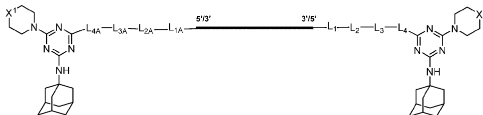
Formula (I''-a-1)
