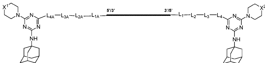
Formula (I''-a-1)
