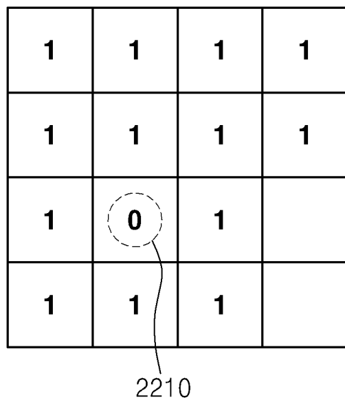
coeff_abs_level_greater1_flag (2200)
