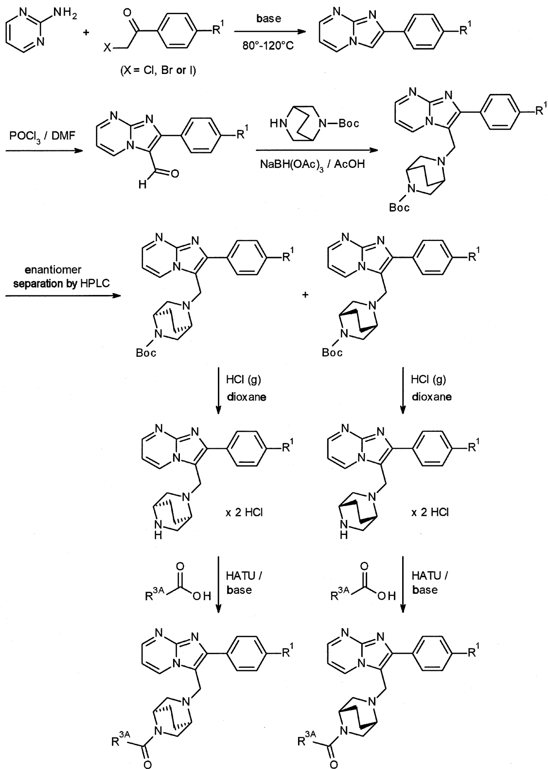
Scheme 1
