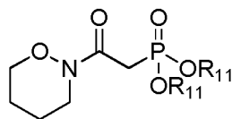
Formula (V)
