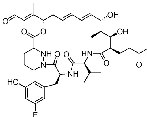
Formula (VI)
