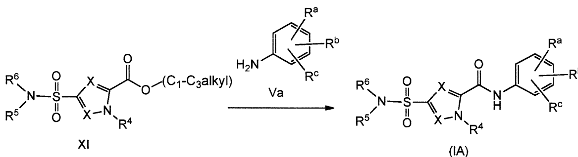
Scheme 5
