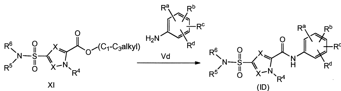
Scheme 5a
