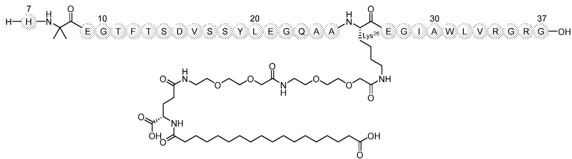
Amino Acid Sequence of Semaglutide
