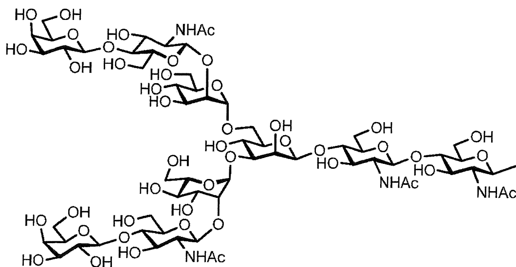
[Chemical Formula 8]
