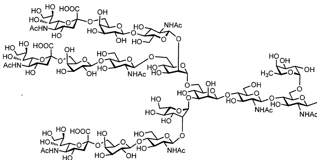
[Chemical Formula -8]
