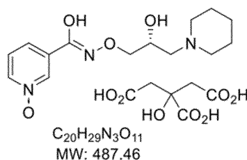
By-product “Hydrolized ORZY-04”
