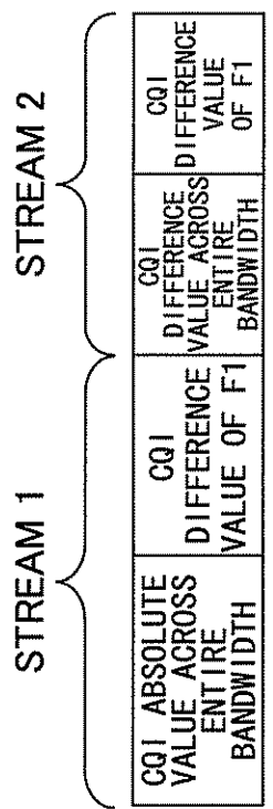
FIG.5B CQI BITS CONFIGURATION IN CQI TTI (CASE 1)
