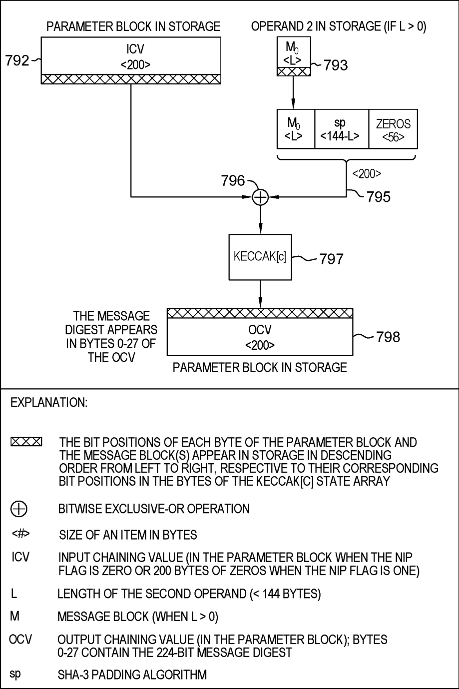
KLMD-SHA3-224 PROCESSING (L < 144)
