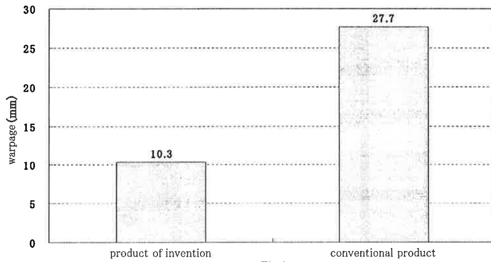
Fig.1 Comparison of Warpage
