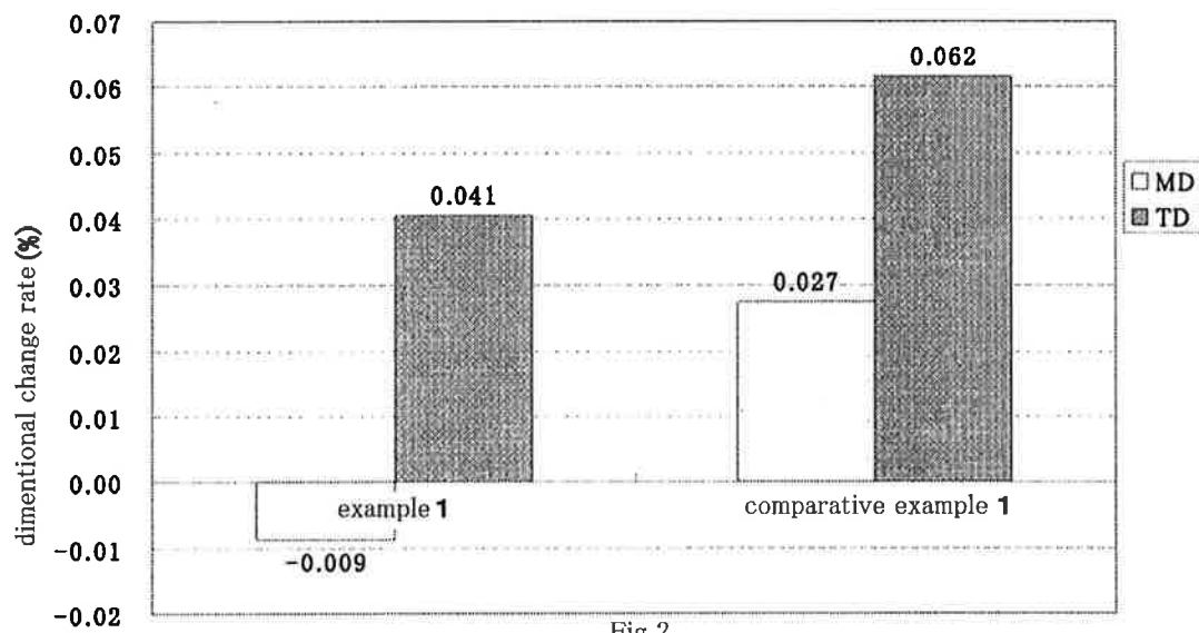
Fig.2 Dimensional Change Rate of Method B
