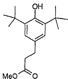
IRGANOX® 1300 (HP)
