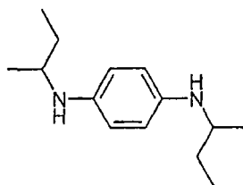
N,N'-Di-sec-butyl-1,4-phenylenediamine (DBPDA)
