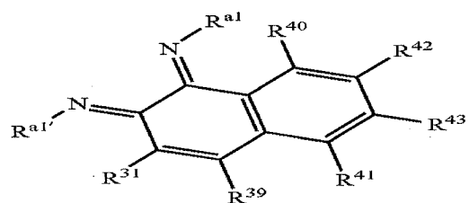
Structure 10f
