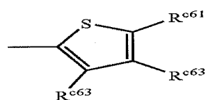
Structure 20c
