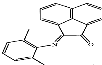
\alpha -Acylimine Compound III
