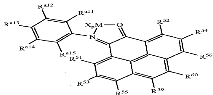
Structure 39d
