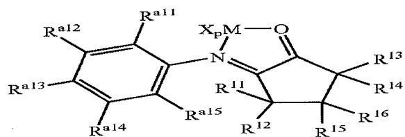
Structure 30d
