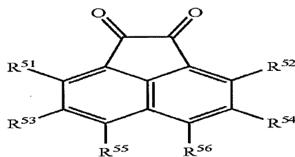
Structure 10
