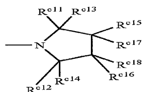
Structure 5c
