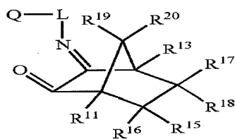
Structure 19b
