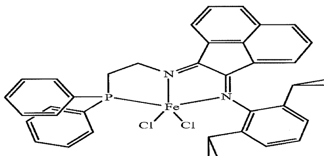
Structure III
