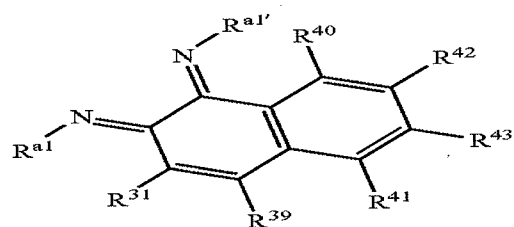
Structure 9f
