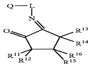
Structure 17b
