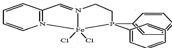
Structure XX
