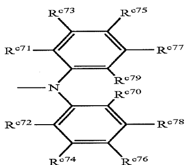
Structure 21c
