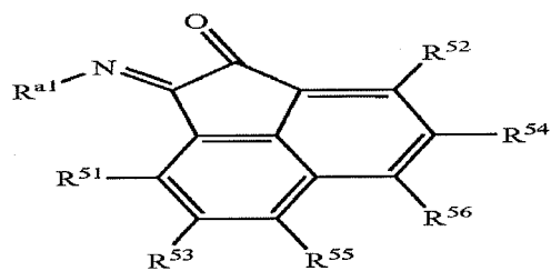
Structure 11b
