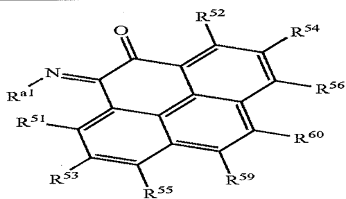
Structure 13b
