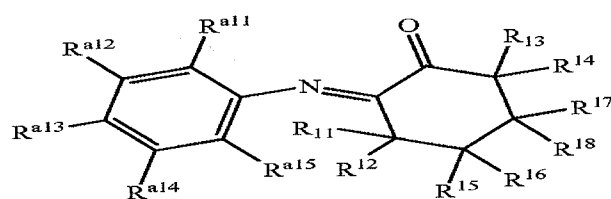
Structure 31b
