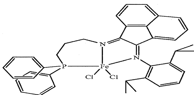
Structure XV
