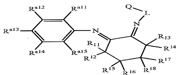
Structure 31f
