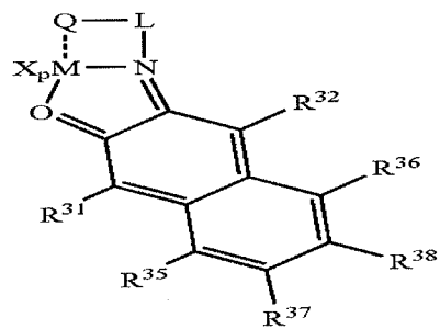
Structure 21d
