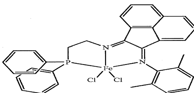
Structure IV
