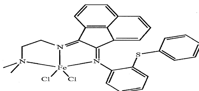
Structure XVI
