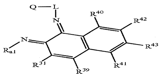
Structure 22f
