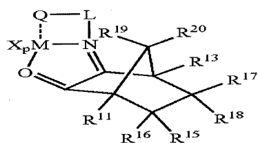
Structure 19d
