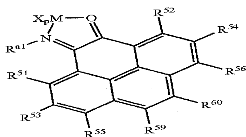
Structure 13d
