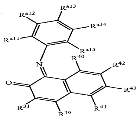
Structure 36b
