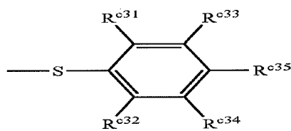
Structure 15c
