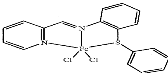
Structure XVIII
