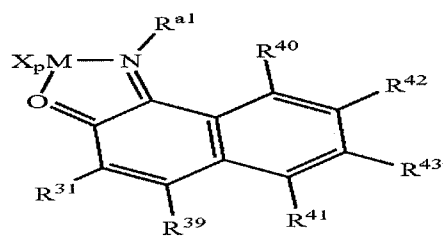
Structure 10d
