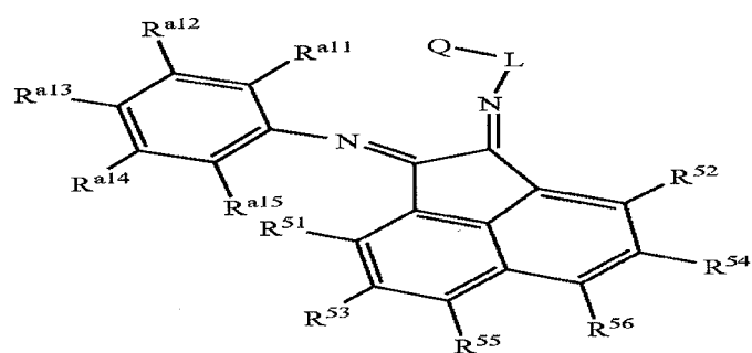
Structure 37f
