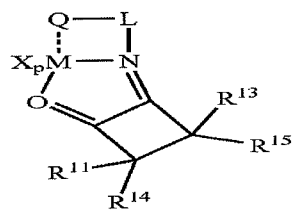
Structure 16d
