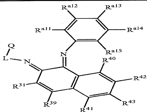
Structure 36f
