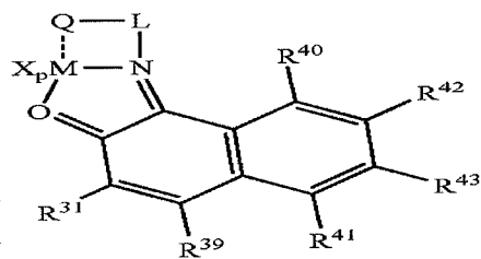
Structure 22d
