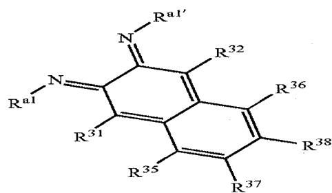
Structure 8f
