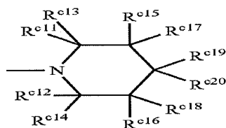
Structure 6c
