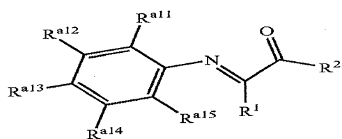
Structure 27b
