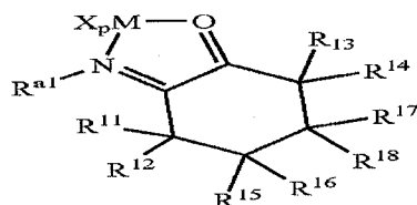
Structure 5d
