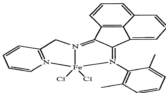
Structure I
