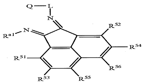
Structure 24f
