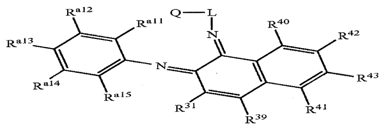
Structure 35f
