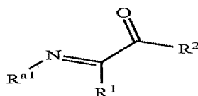
Structure 1b
