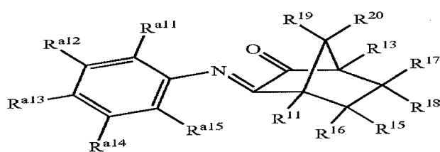
Structure 32b
