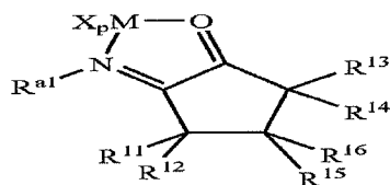
Structure 4d
