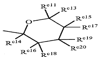
Structure 13c
