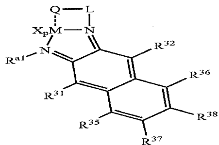
Structure 21e
