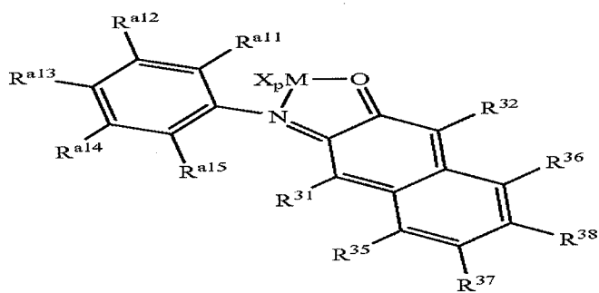
Structure 34d
