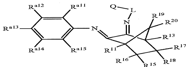
Structure 32f
