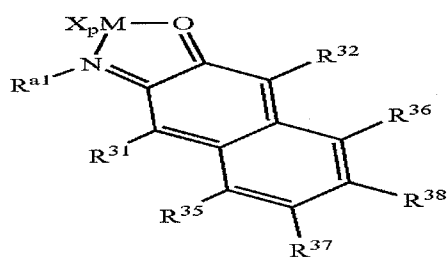
Structure 8d
