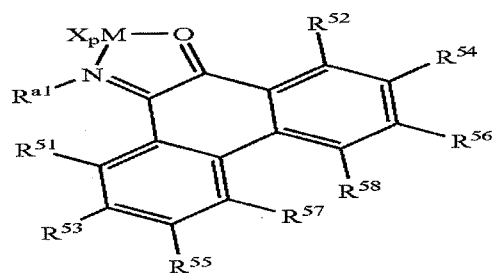
Structure 12d
