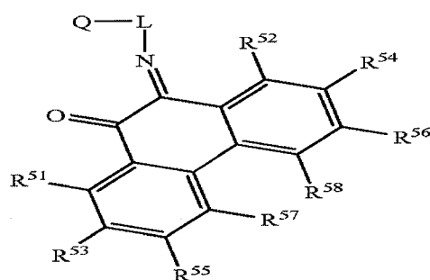
Structure 25b
