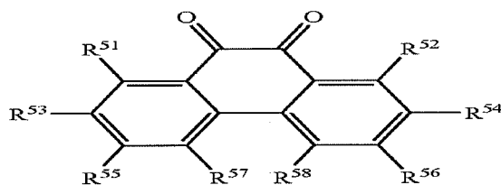
Structure 11
