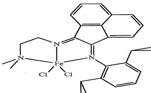
Structure XI
