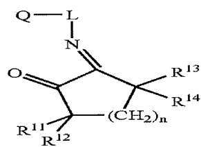
Structure 15b
