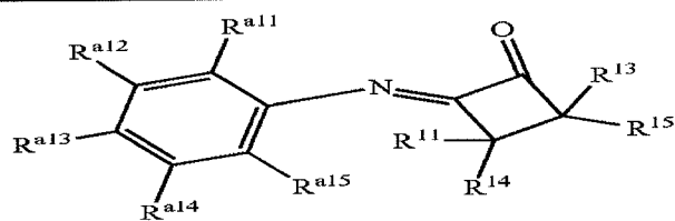
Structure 29b
