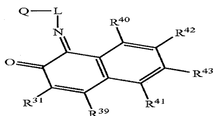
Structure 22b
