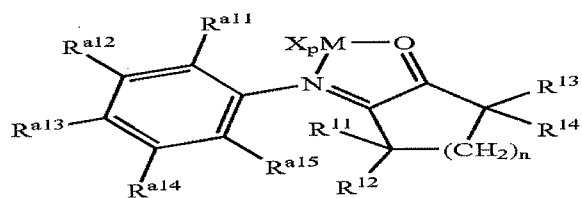
Structure 28d
