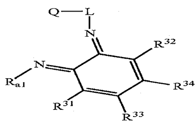
Structure 20f
