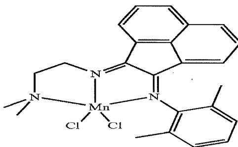
Structure XXII
