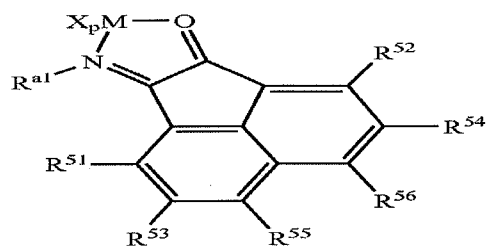
Structure 11d
