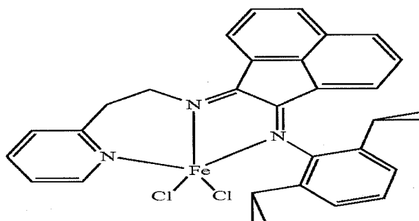
Structure VIII
