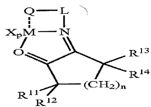
Structure 15d
