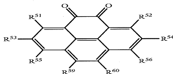
Structure 12
