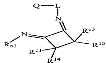
Structure 16f
