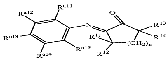
Structure 28b
