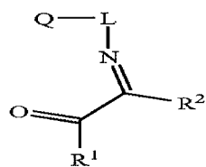
Structure 14b
