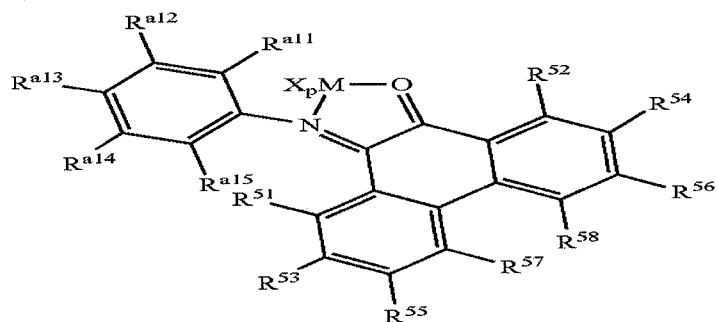
Structure 38d
