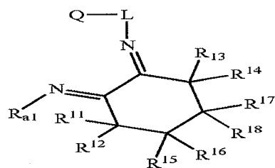
Structure 18f
