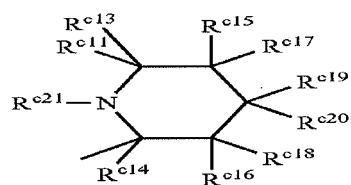
Structure 9c
