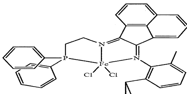
Structure XIV
