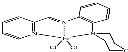
Structure XIX
