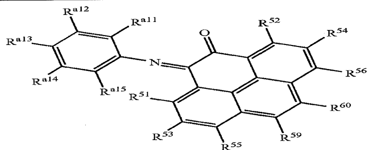
Structure 39b
