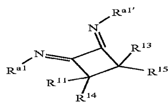
Structure 3f
