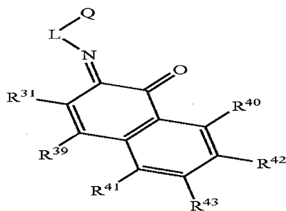
Structure 23b
