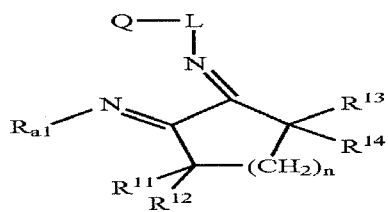
Structure 15f
