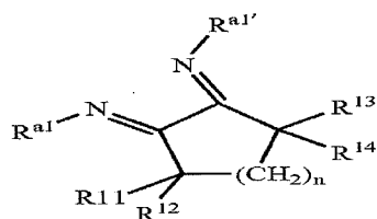
Structure 2f
