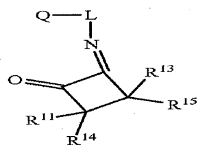
Structure 16b
