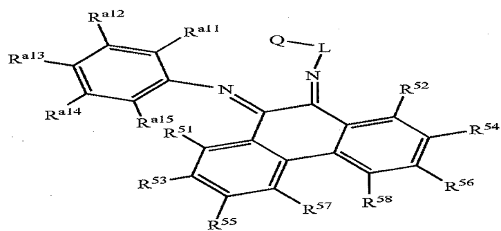
Structure 38f
