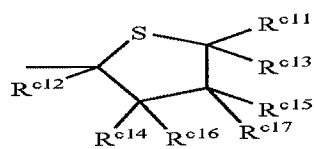
Structure 12c
