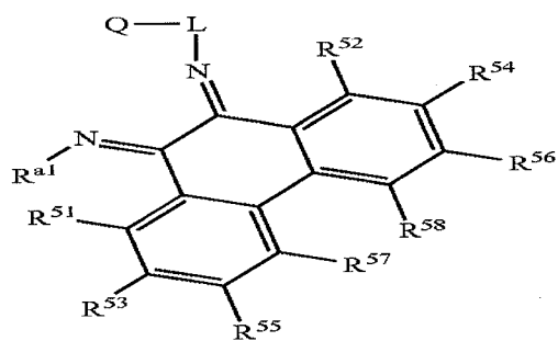
Structure 25f
