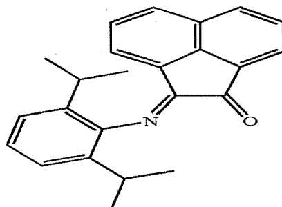
\alpha -Acylimine Compound I
