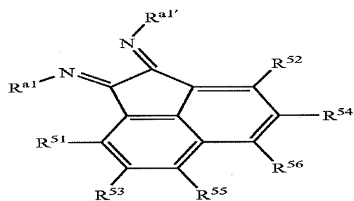
Structure 11f
