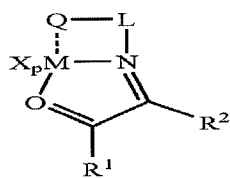
Structure 14d
