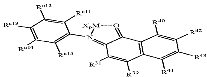
Structure 35d
