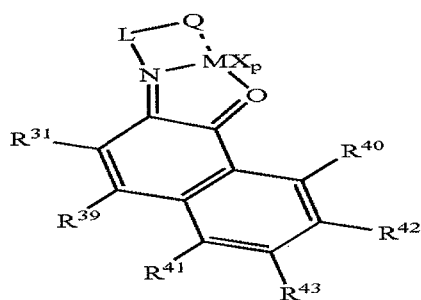
Structure 23d
