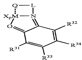
Structure 20d
