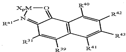
Structure 9d
