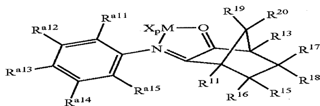
Structure 32d
