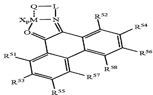
Structure 25d
