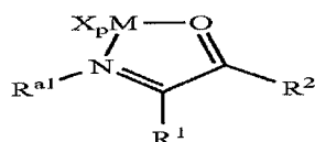
Structure 1d
