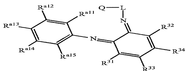
Structure 33f
