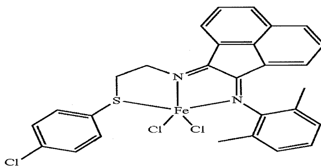
Structure V
