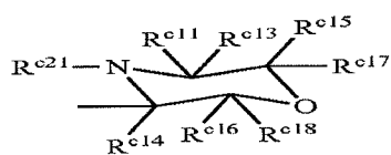
Structure 10c
