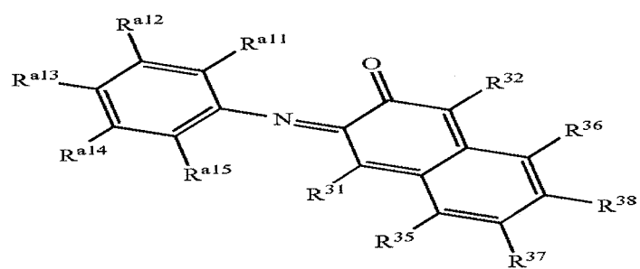
Structure 34b
