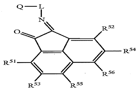
Structure 24b
