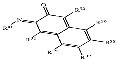
Structure 8b
