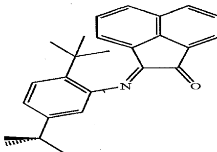
\alpha -Acylimine Compound II
