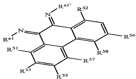
Structure 12f
