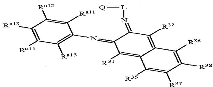
Structure 34f
