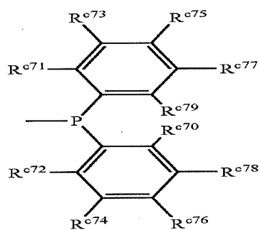
Structure 22c
