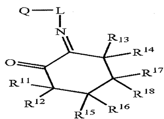
Structure 18b
