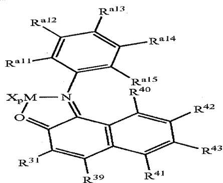
Structure 36d
