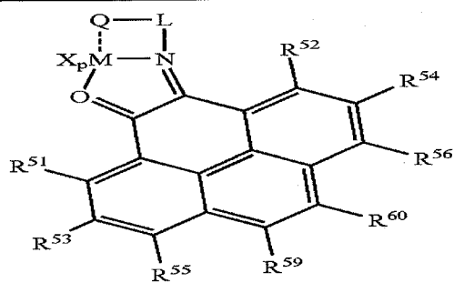
Structure 26d
