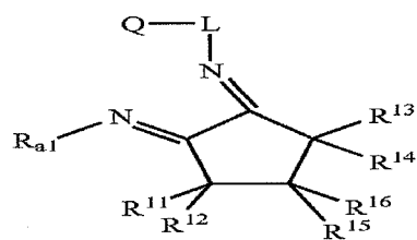
Structure 17f
