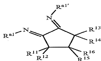
Structure 4f
