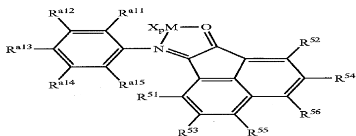
Structure 37d
