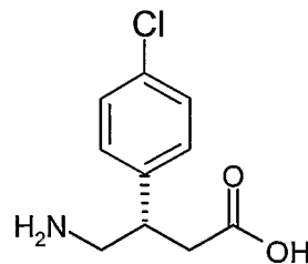
S-Baclofen (3)
