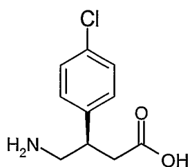
R-Baclofen (2)
