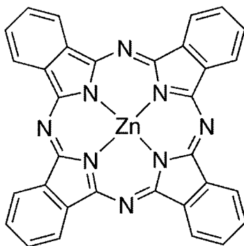
[0062] zinc phthalocyanine:
