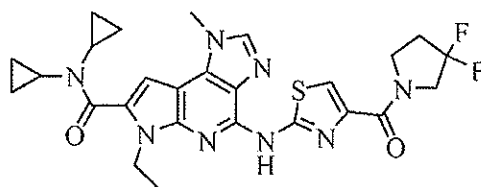
N,N -dicyclopropyl-4-(4-(3,3-difluoropyrrolidine-1-carbonyl)thiazol-2-ylamino)- 6-ethyl-1-methyl-1,6-dihydroimidazo[4,5-d]pyrrolo[2,3-b]pyridine-7- carboxamide
