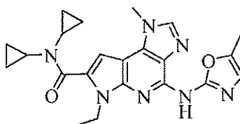
N,N -dicyclopropyl-6-ethyl-1-methyl-4-(5-methyloxazol-2-ylamino)-1,6-dihydroimidazo[4,5-d]pyrrolo[2,3-b]pyridine-7-carboxamide
