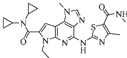
2-(7-(dicyclopropylcarbamoyl)-6-ethyl-1-methyl-1,6-dihydroimidazo[4,5-d]pyrrolo[2,3-b]pyridin-4-ylamino)-N,4-dimethylthiazole-5-carboxamide
