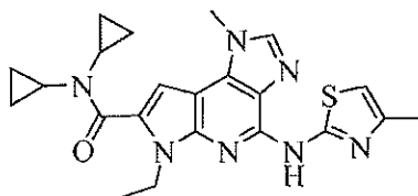
N,N -dicyclopropyl-6-ethyl-1-methyl-4-(4-methylthiazol-2-ylamino)-1,6-dihydroimidazo[4,5-d]pyrrolo[2,3-b]pyridine-7-carboxamide
