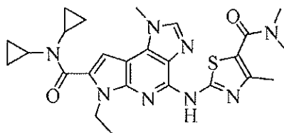
2-(7-(dicyclopropylcarbamoyl)-6-ethyl-1-methyl-1,6-dihydroimidazo[4,5-d]pyrrolo[2,3-b]pyridin-4-ylamino)- N,N ,4-trimethylthiazole-5-carboxamid
