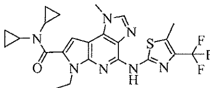
Preparation of N,N -dicyclopropyl-6-ethyl-1-methyl-4-(5-methyl-4-(trifluoromethyl)thiazol-2-ylamino)-1,6-dihydroimidazo[4,5-d]pyrrolo[2,3-b]pyridine-7-carboxamide
