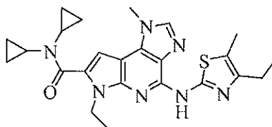
N,N -dicyclopropyl-6-ethyl-4-(4-ethyl-5-methylthiazol-2-ylamino)-1-methyl-1,6-dihydroimidazo[4,5-d]pyrrolo[2,3-b]pyridine-7-carboxamide
