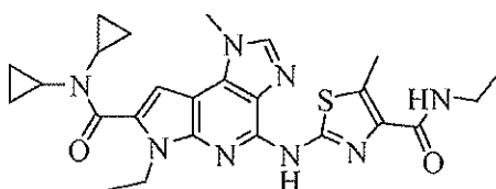
15 2-(7-(dicyclopropylcarbamoyl)-6-ethyl-1-methyl-1,6-dihydroimidazo[4,5-d]pyrrolo[2,3-b]pyridine-4-ylamino)-N-ethyl-5-methylthiazole-4-carboxamide
