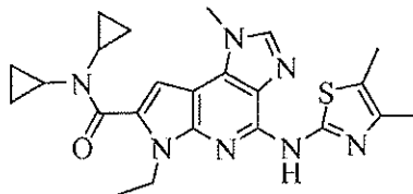
N,N -dicyclopropyl-4-(4,5-dimethylthiazol-2-ylamino)-6-ethyl-1-methyl-1,6-dihydroimidazo[4,5-d]pyrrolo[2,3-b]pyridine-7-carboxamide
