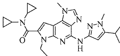
N,N -dicyclopropyl-6-ethyl-4-(5-isopropyl-1-methyl-1 H -pyrazol-3-ylamino)-1-methyl-1,6-dihydroimidazo[4,5- d ]pyrrolo[2,3- b ]pyridine-7-carboxamide
