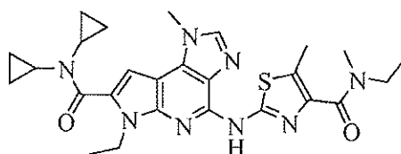
2-(7-(dicyclopropylcarbamoyl)-6-ethyl-1-methyl-1,6-dihydroimidazo[4,5-d]pyrrolo[2,3-b]pyridin-4-ylamino)-N-ethyl-N,5-dimethylthiazole-4-carboxamide
