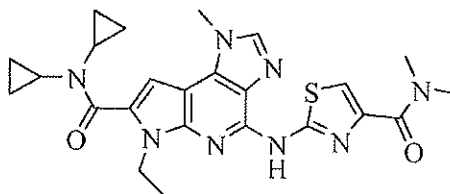
2-(7-(dicyclopropylcarbamoyl)-6-ethyl-1-methyl-1,6-dihydroimidazo[4,5-d]pyrrolo[2,3-b]pyridin-4-ylamino)- N,N -dimethylthiazole-4-carboxamide
