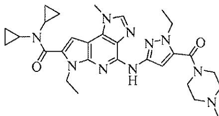
N,N -dicyclopropyl-6-ethyl-4-(1-ethyl-5-(4-methylpiperazine-1-carbonyl)-1 H -pyrazol-3-ylamino)-1-methyl-1,6-dihydroimidazo[4,5- d ]pyrrolo[2,3- b ]pyridine-7-carboxamide
