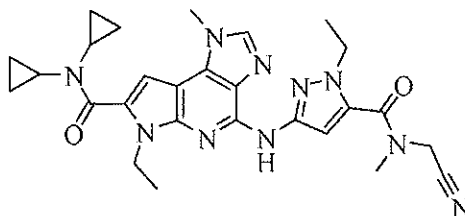
4-(5-((cyanomethyl)(methyl)carbamoyl)-1-ethyl-1 H -pyrazol-3-ylamino)- N,N -dicyclopropyl-6-ethyl-1-methyl-1,6-dihydroimidazo[4,5- d ]pyrrolo[2,3- b ]pyridine-7-carboxamide
