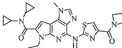
(4-(azetidine-1-carbonyl)thiazol-2-ylamino)- N,N -dicyclopropyl-6-ethyl-1-methyl- 1,6-dihydroimidazo[4,5-d]pyrrolo[2,3-b]pyridine-7-carboxamide
