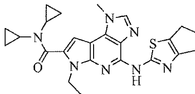
N,N -dicyclopropyl-4-(5,6-dihydro-4H-cyclopenta[d]thiazol-2-ylamino)-6-ethyl-1-methyl-1,6-dihydroimidazo[4,5-d]pyrrolo[2,3-b]pyridine-7-carboxamide
