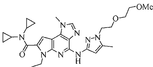
N,N -dicyclopropyl-6-ethyl-4-(1-(2-(2-methoxyethoxy)ethyl)-5-methyl-1 H -pyrazol-3-ylamino)-1-methyl-1,6-dihydroimidazo[4,5- d ]pyrrolo[2,3- b ]pyridine-7-carboxamide
