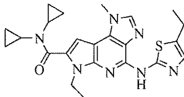
N,N -dicyclopropyl-6-ethyl-4-(5-ethylthiazol-2-ylamino)-1-methyl-1,6-dihydroimidazo[4,5-d]pyrrolo[2,3-b]pyridine-7-carboxamide
