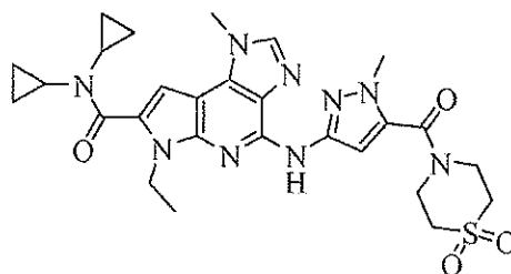
N,N -dicyclopropyl-6-ethyl-4-(1-methyl-5-(thiomorpholine 1,1-dioxide-4-carbonyl)-1 H -pyrazol-3-ylamino)-1-methyl-1,6-dihydroimidazo[4,5-d]pyrrolo[2,3-b]pyridine-7-carboxamide
