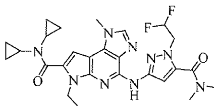
N,N -dicyclopropyl-4-(1-(2,2-difluoroethyl)-5-(dimethylcarbamoyl)-1 H -pyrazol-3-ylamino)-6-ethyl-1-methyl-1,6-dihydroimidazo[4,5-d]pyrrolo[2,3-b]pyridine-7-carboxamide
