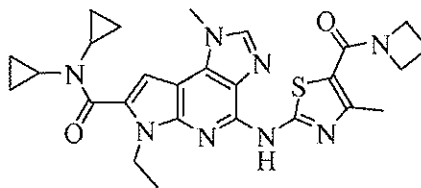
4-(5-(azetidine-1-carbonyl)-4-methylthiazol-2-ylamino)-N,N-dicyclopropyl-6-ethyl-1-methyl-1,6-dihydroimidazo[4,5-d]pyrrolo[2,3-b]pyridine-7-carboxamide
