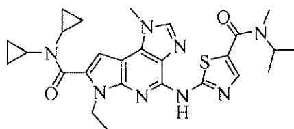
2-(7-(dicycloppropylcarbamoyl)-6-ethyl-1-methyl-1,6-dihydroimidazo[4,5-d]pyrrolo[2,3-b]pyridin-4-ylamino)-N-isopropyl-N-methylthiazole-5-carboxamide
