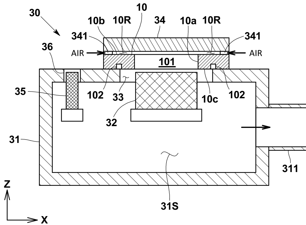
(a) STATE IN WHICH THE FIRST CLEANING BODY IS LOWERED
