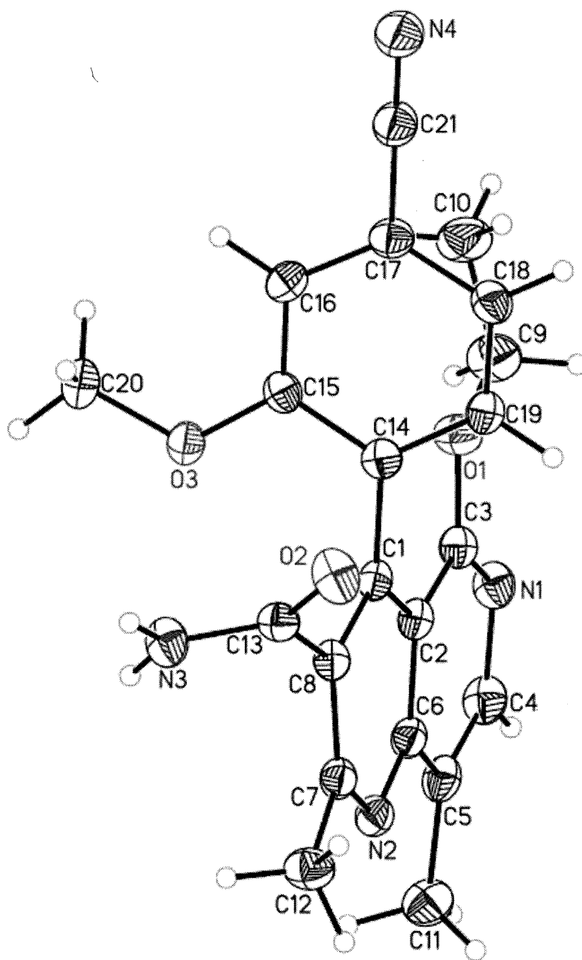
Figure 1: Crystal structure of the compound of the formula M1b (R): (R)-4-(4-cyano-2-methoxyphenyl)-5-ethoxy-2,8-dimethyl-1,6-naphthyridine-3-carboxamide
