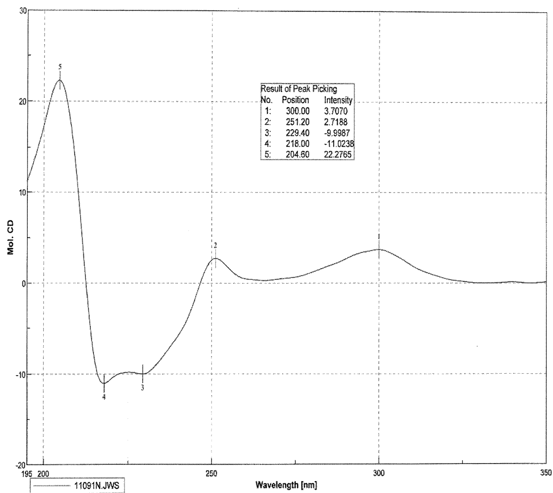
Figure 3: CD spectrum of the compound of the formula M1b (R) (in acetonitrile)
