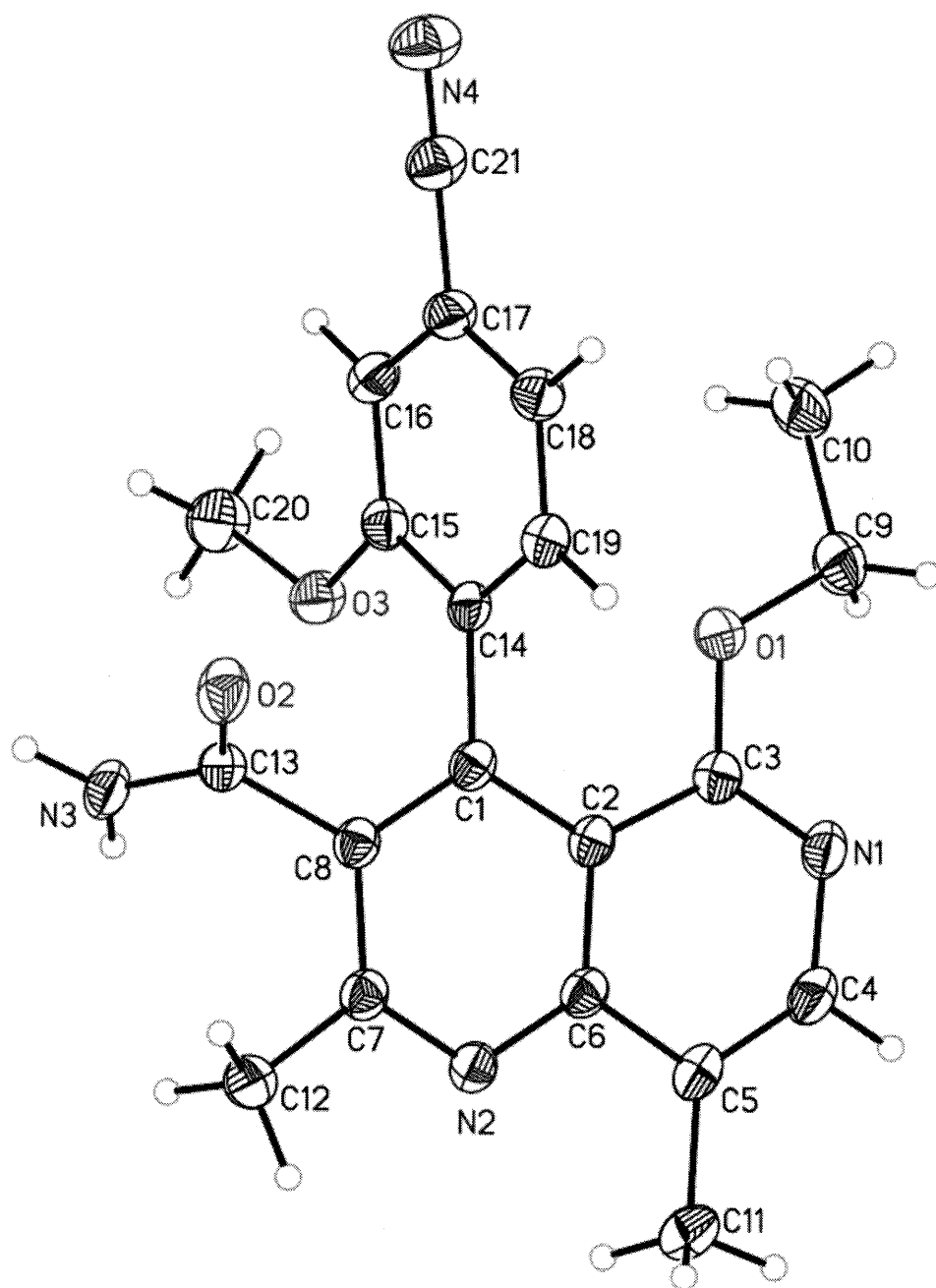
Figure 2: Crystal structure of the compound of the formula M1b (R): (R)-4-(4-cyano-2-methoxyphenyl)-5-ethoxy-2,8-dimethyl-1,6-naphthyridine-3-carboxamide
