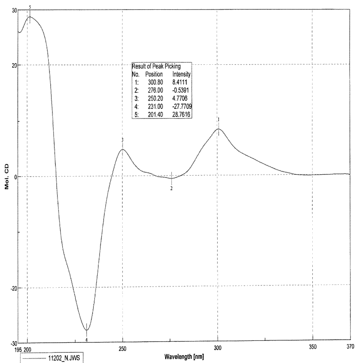
Figure 5: CD spectrum of the compound of the formula M3b (R) (in acetonitrile)
