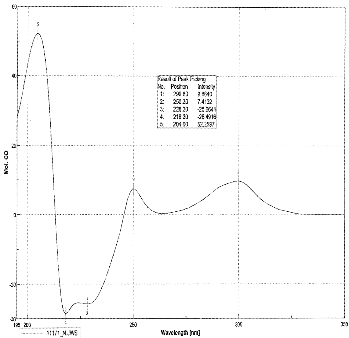
Figure 4: CD spectrum of the compound of the formula M2b (R) (in acetonitrile)
