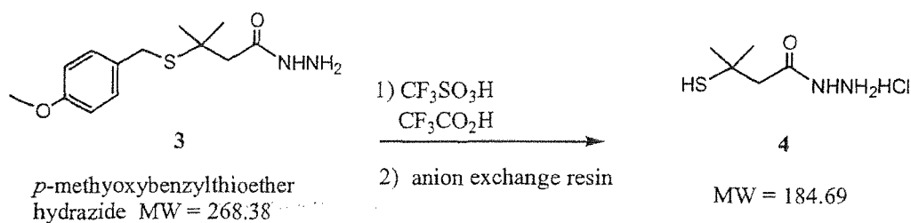
Equation V
