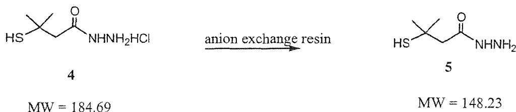
Equation V
