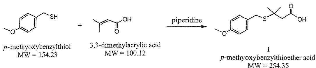
Equation I
