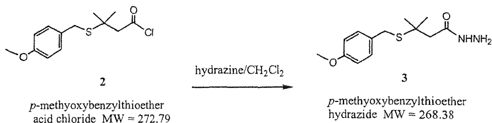
Equation III
