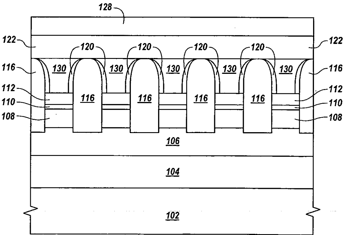
X-X Section
