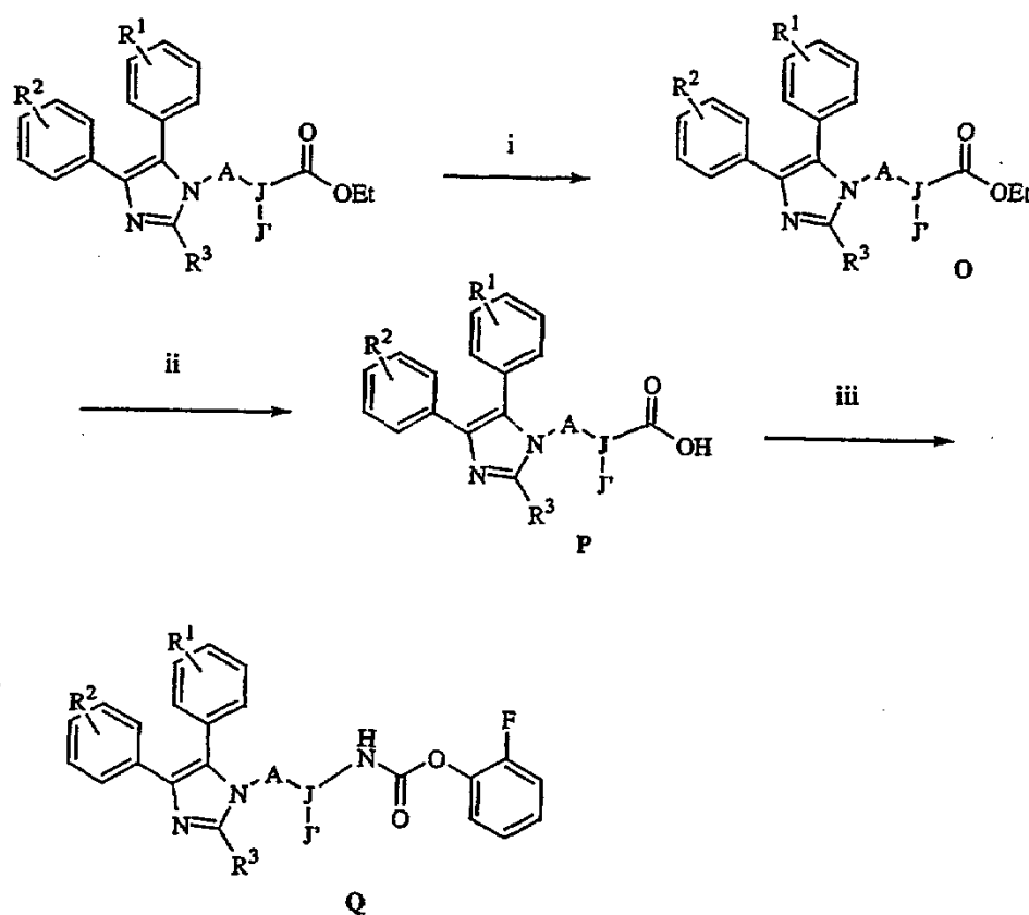
Scheme 3. Reaction conditions: (i) [(CH_3)_3Si]_2NNa , THF, R_5I , -78^\circ C to rt; (ii) NaOH, MeOH, Reflux; (iii) (a) N_3P(O)(OPh)_2 , Et_3N , toluene, 108^\circ C , (b) 2-fluorophenol, 100^\circ C .
