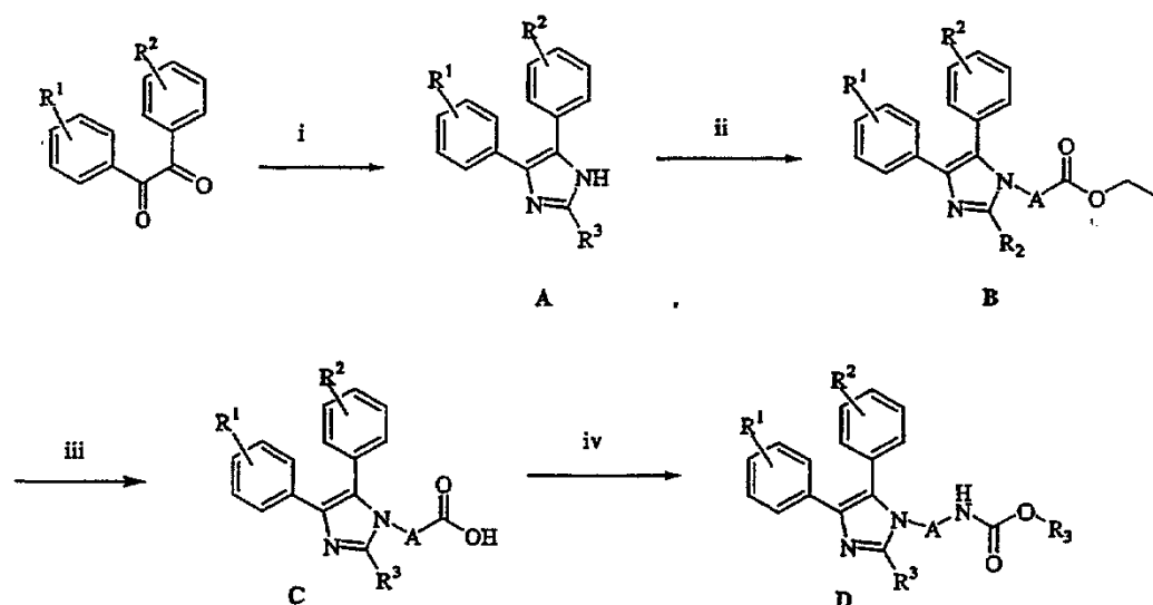
Scheme 1. Reaction conditions: (i) aldehyde, CH 3 COONH 4 , CH 3 COOH, 100 °C; (ii) bromide, NaH, DMF, rt; (iii) NaOH, EtOH, rt; (iv) (a) N 3 P(O)(OPh) 2 , Et 3 N, toluene, 105 °C, (b) R 3 OH, 80 °C.
