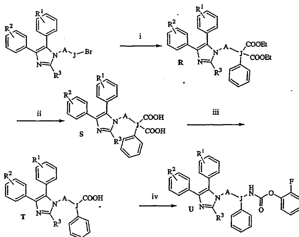
Scheme 4. Reaction conditions: (i) (a) NaH, DMF, rt, (b) diethyl phenyl malonate, 45-50 °C (ii) NaOH, THF, 80 °C; (iii) CH 3 COOH, reflux; (iv) (a) N 3 P(O)(OPh) 2 , Et 3 N, toluene, 108 °C, (b) 2-fluorophenol, 100 °C.
