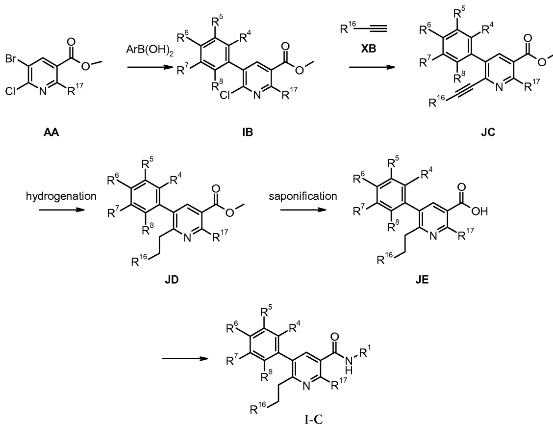
Scheme 10
