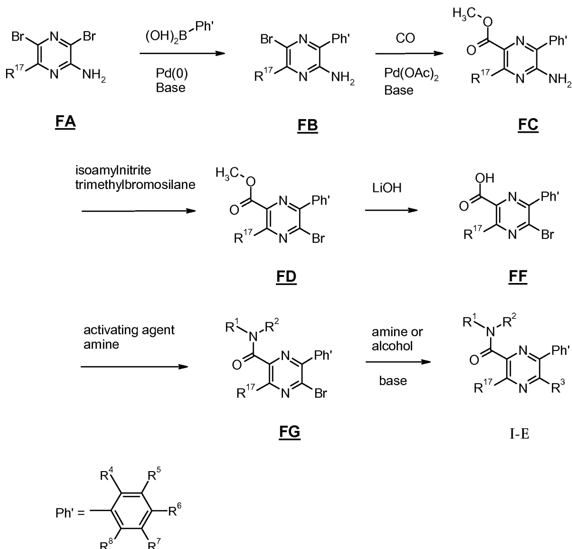
Scheme 6
