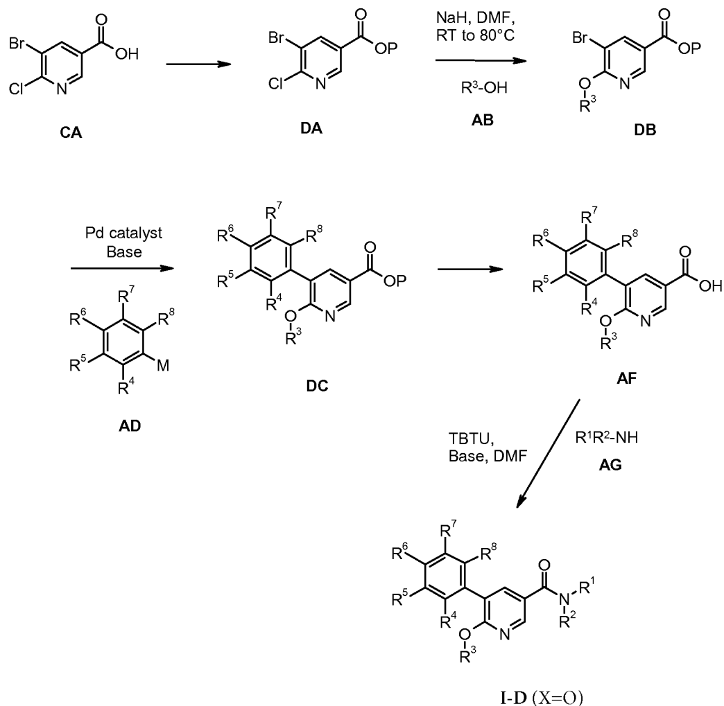
Scheme 4
