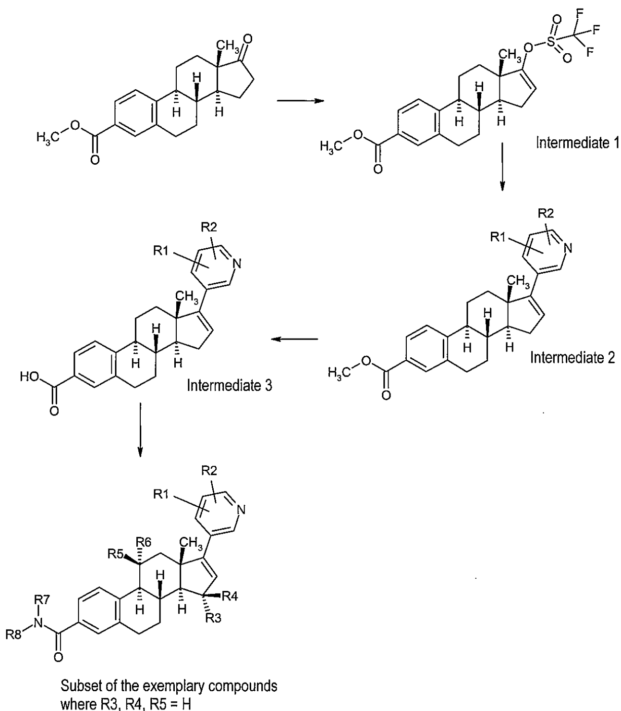
Synthesis scheme 1
