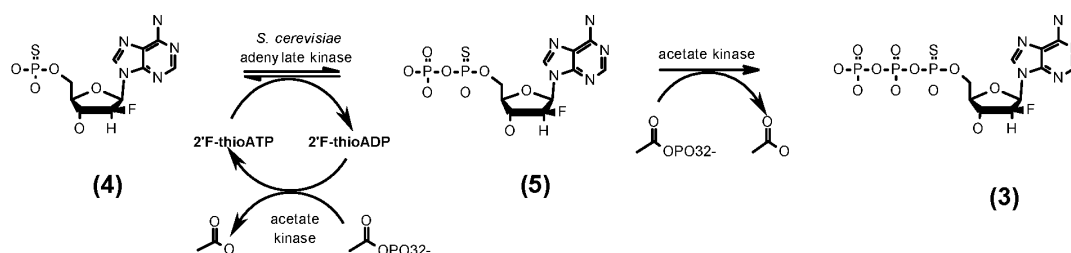
Scheme 3: Production of F-thioATP Compound (3) by Adenylate Kinase and Acetate Kinase
