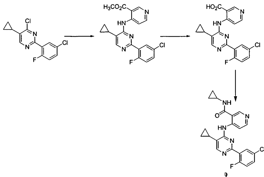
Scheme 9
