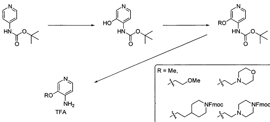
Scheme 6
