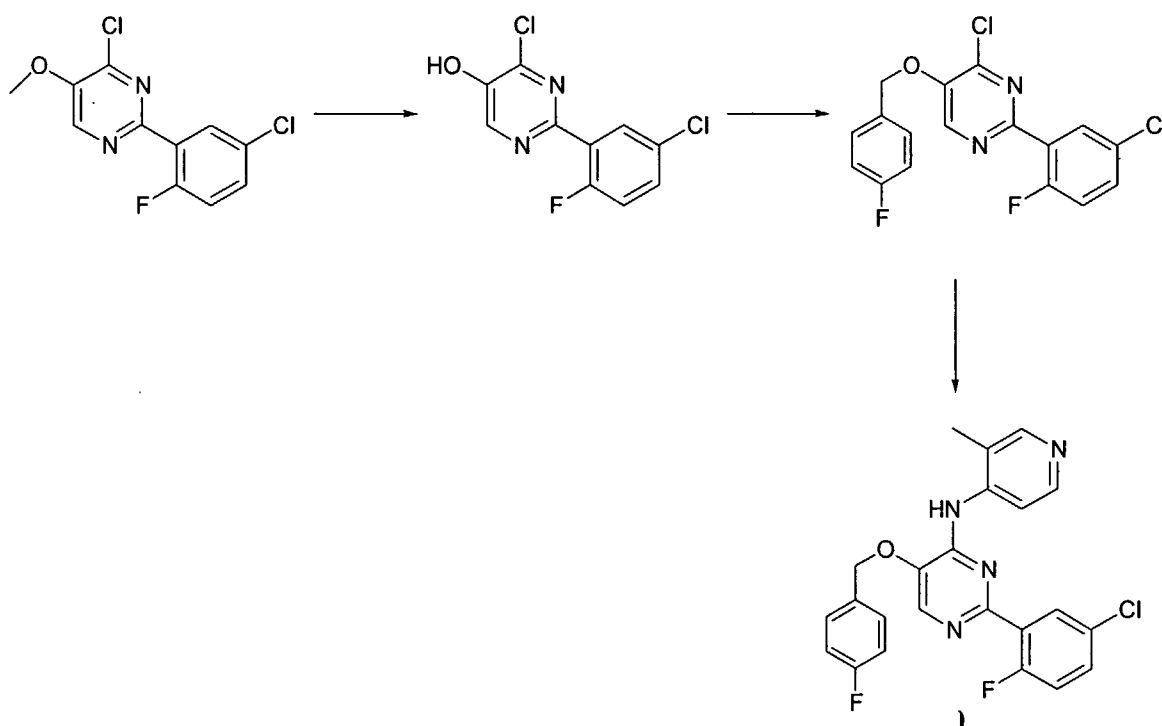
Scheme 13a
