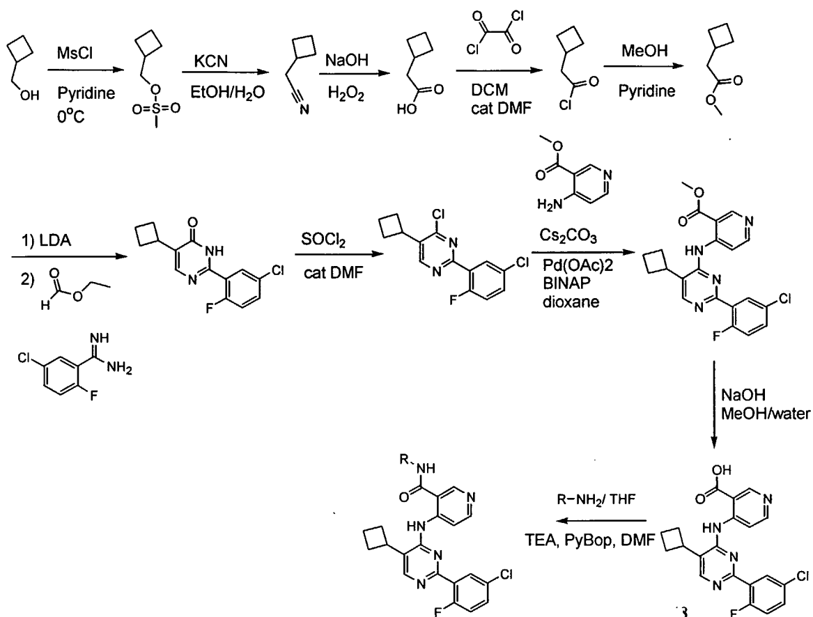
Scheme 10
