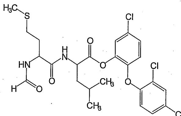
Compound # 2
