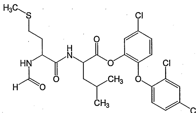
Compound # 2
