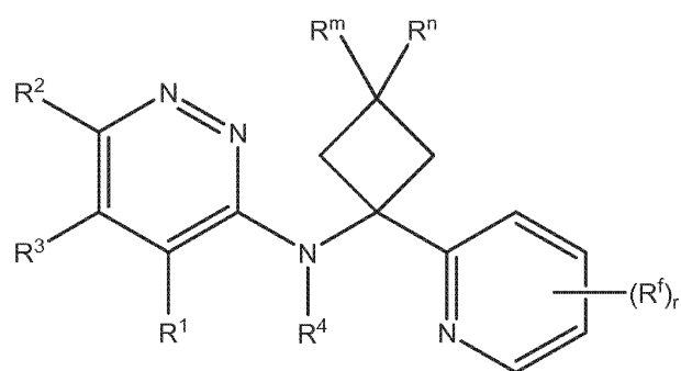
Formula XII(n)
