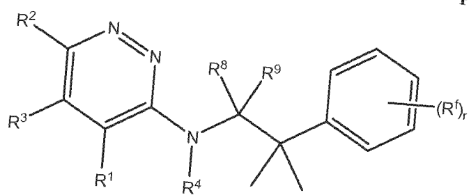
Formula XII(h)
