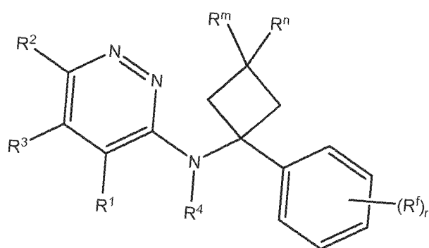
Formula XII(i)
