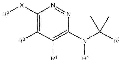
Formula IV(a)
