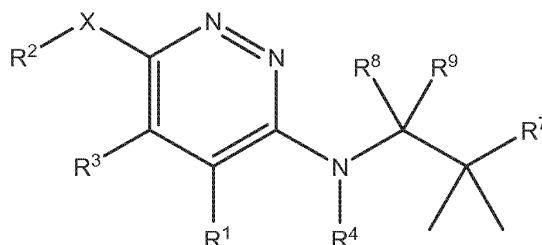
Formula IV(b)
