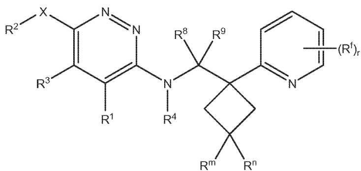
Formula XI(b)
