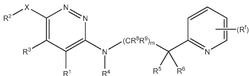
Formula IX
