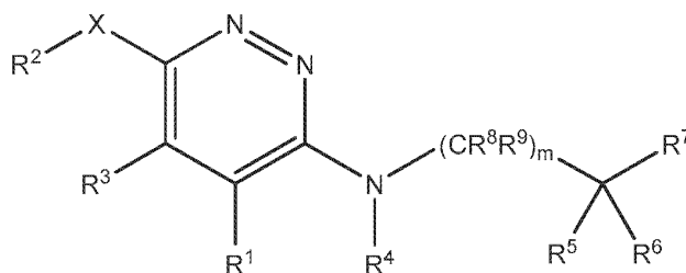
Formula I
