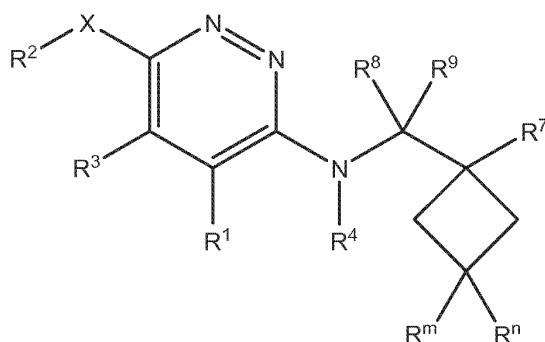
Formula V(b)
