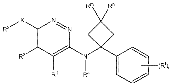
Formula VIII(a)
