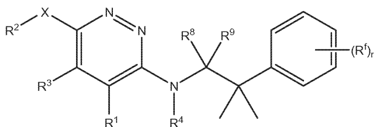
Formula VII(b)
