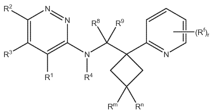
Formula XII(o)
