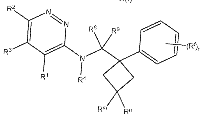
Formula XII(j)
