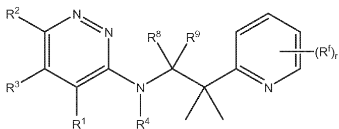
Formula XII(m)
