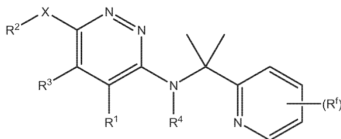
Formula X(a)
