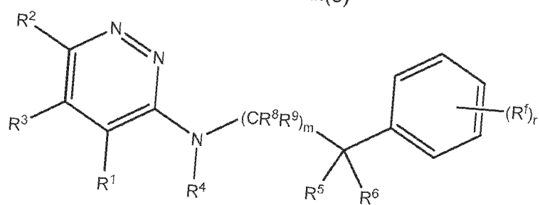
Formula XII(f)
