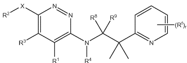
Formula X(b)
