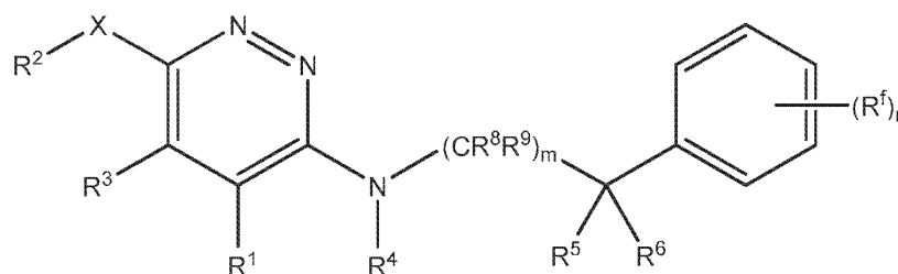
Formula VI
