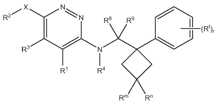
Formula VIII(b)
