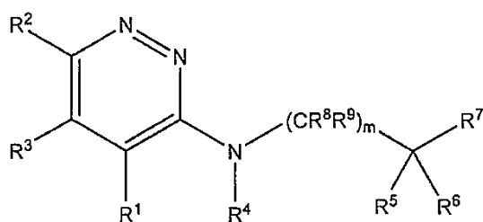
Formula XII(a)
