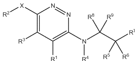
Formula III
