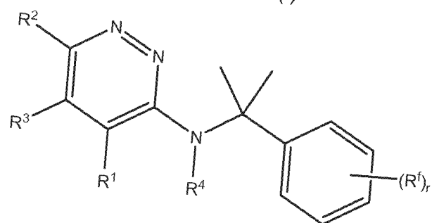
Formula XII(g)
