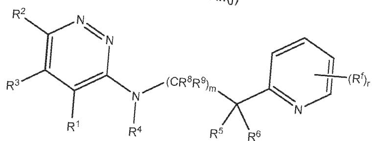
Formula XII(k)
