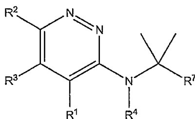
Formula XII(b)
