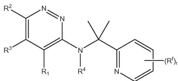
Formula XII(l)
