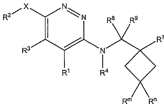
Formula V(a)
