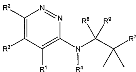
Formula XII(c)
