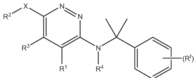
Formula VII(a)
