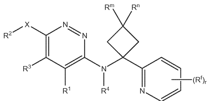
Formula XI(a)
