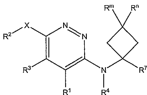
Formula V(a)
