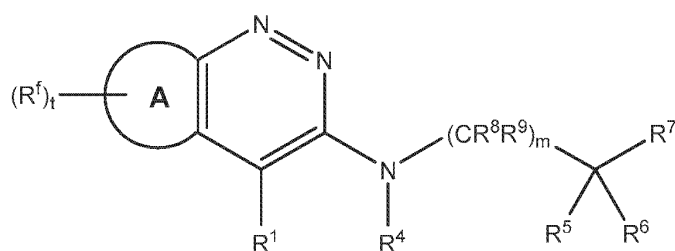
Formula XIII
