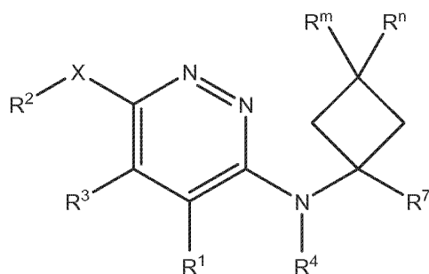
Formula V(a)
