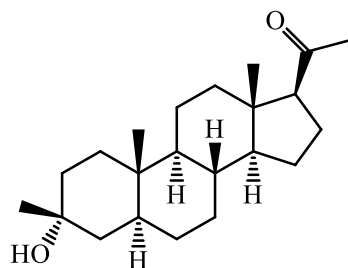
3 \alpha -hydroxy, 3 \beta -methyl-5 \alpha -pregnan-20-one Ganaxolone
