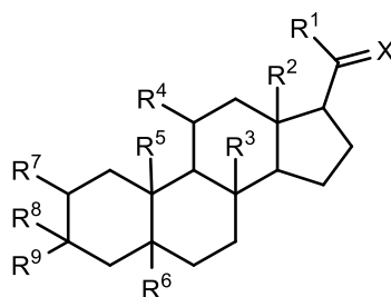
Formula IA
