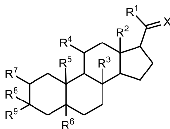
Formula IB
