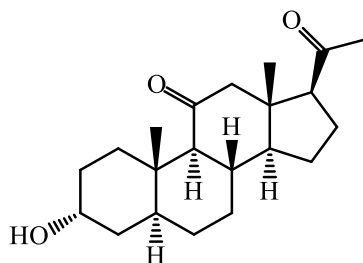
3 \alpha -hydroxy-5 \alpha -pregnane-11,20-dione Alphaxalone
