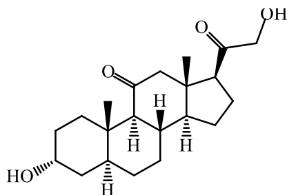
3 \alpha , 21-dihydroxy-5 \alpha -pregnane-11,20-dione Alphadolone
