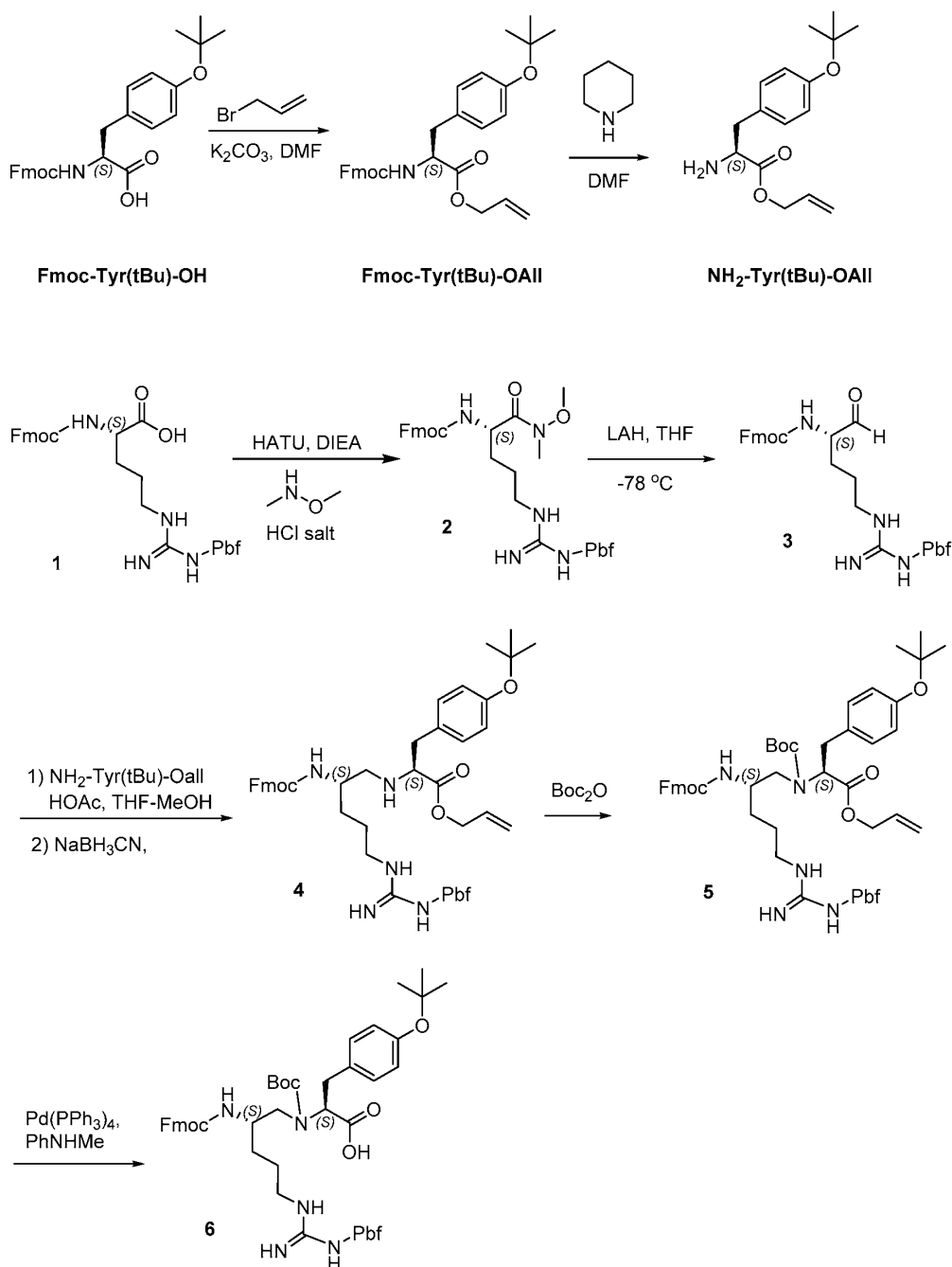
Scheme 14. Synthesis of Fmoc- psi -[Arg(Pbf)-(N-Boc)Tyr(tBu)]-OH
