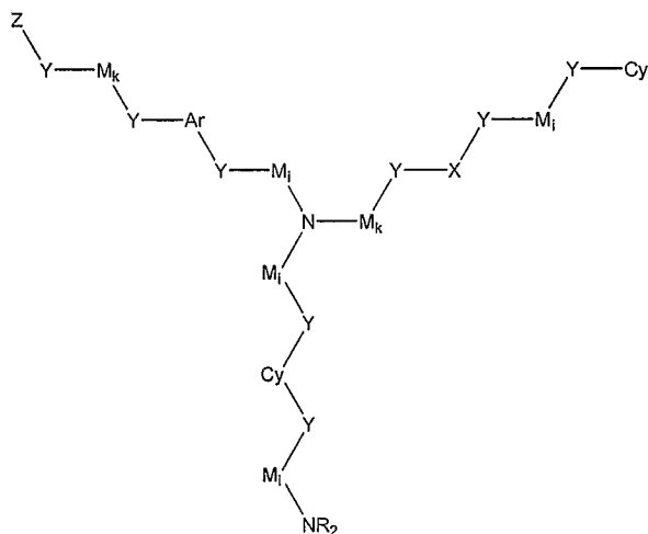
Formula XI
