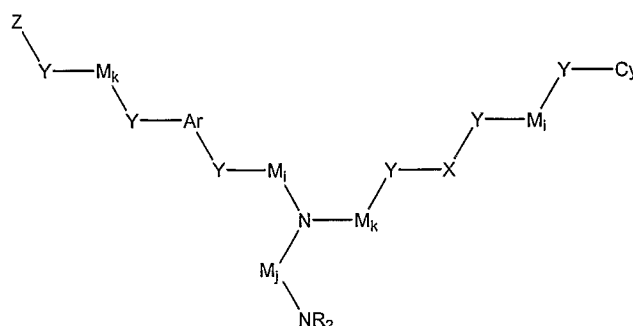
Formula X
