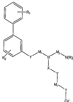
Formula V
