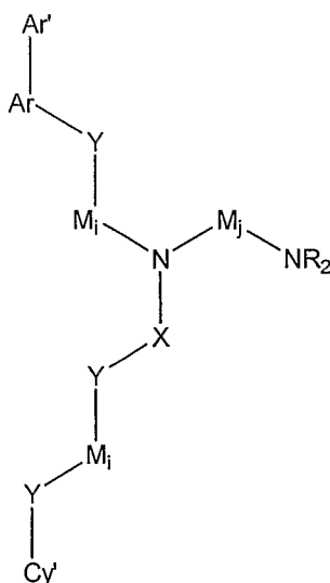
Formula II
