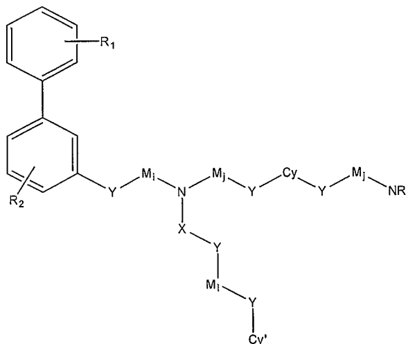
Formula VI
