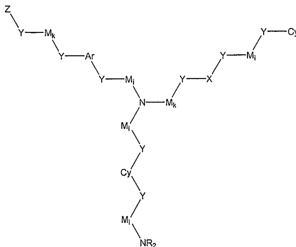
Formula XI
