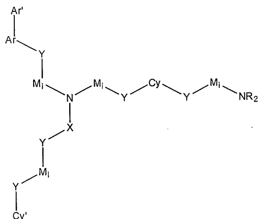
Formula III
