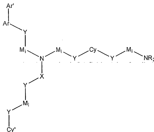
Formula IV
