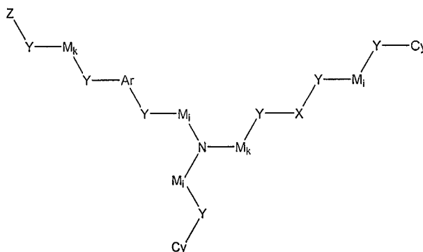
Formula IX
