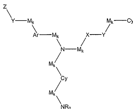
Formula XII
