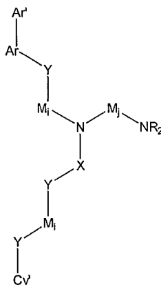
Formula II
