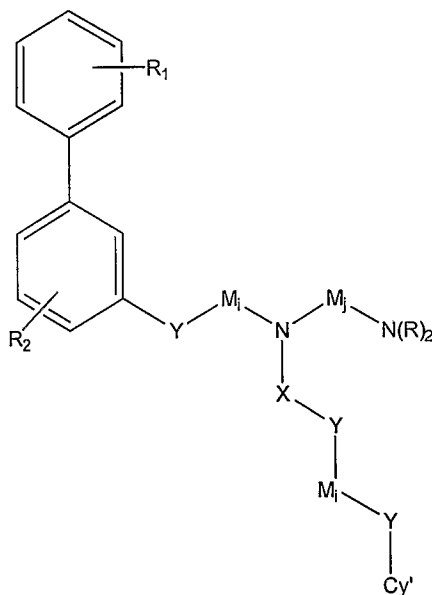
Formula V
