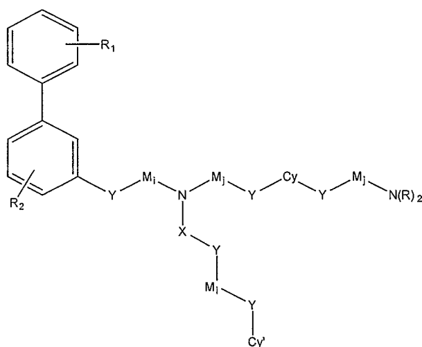
Formula VI
