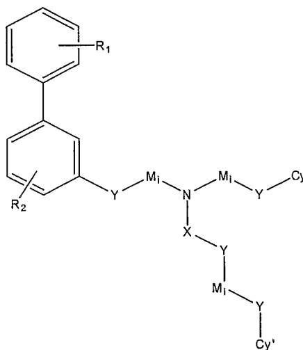
Formula IV
