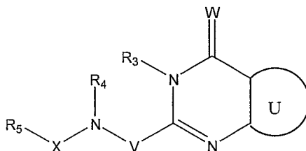
Formula VIII
