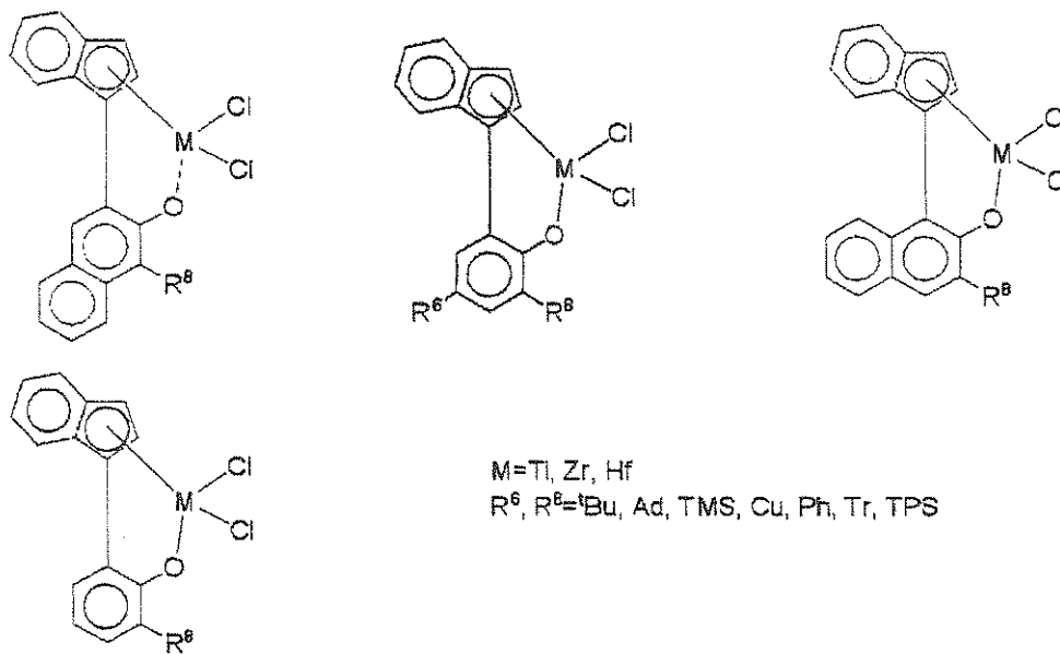
[Chem. 14]
