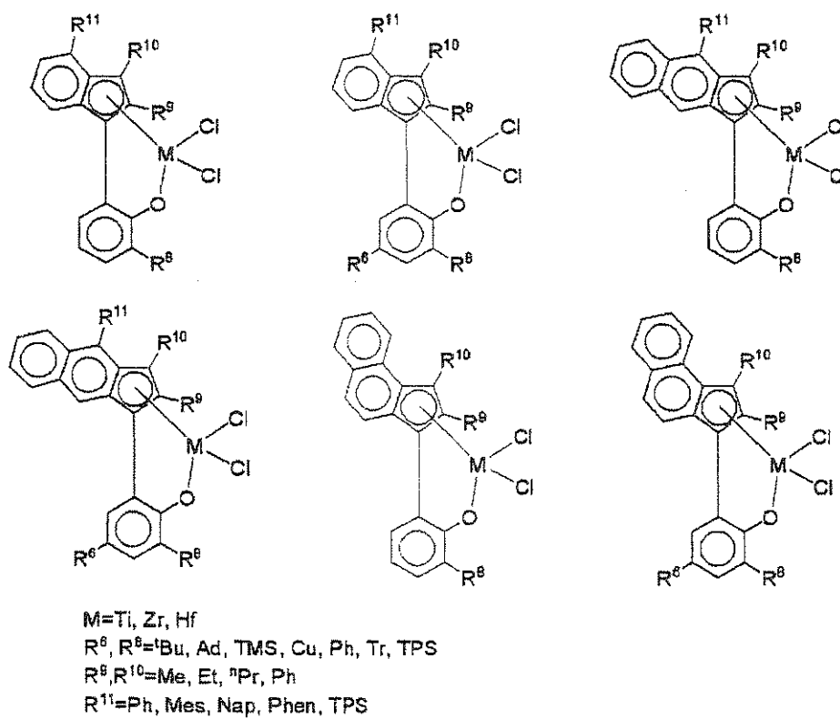
[Chem. 15]
