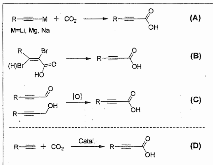
Scheme 2: Protocols for synthesis of substituted propiolic acids.
