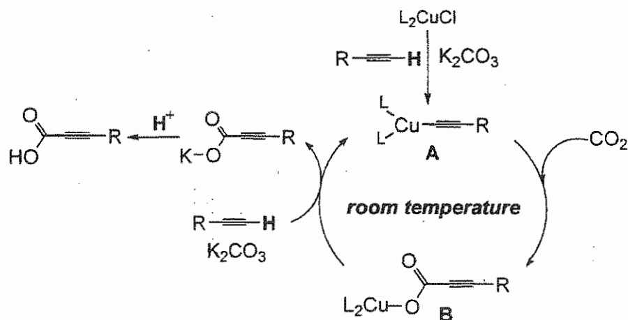
Scheme 4. Proposed catalytic cycle.
