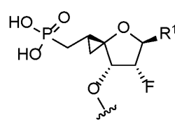
Formula (33)
