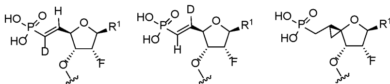
Formula (31)
