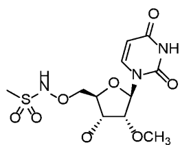
Formula (14A)
