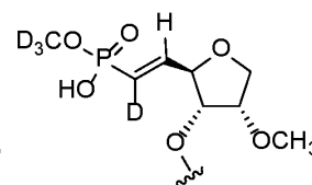
Formula (11BY)
