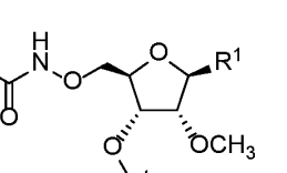
Formula (15)
