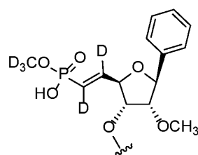
Formula (10AY)
