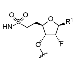
Formula (26)
