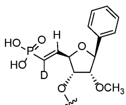
Formula (11A)
