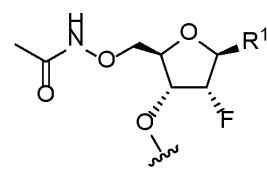
Formula (35)
