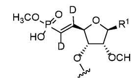
Formula (10X)
