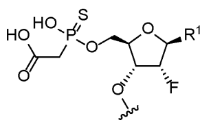
Formula (28)
