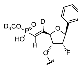
Formula (32AY)
