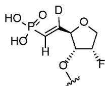
Formula (32B)
