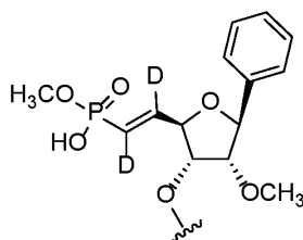
Formula (10AX)
