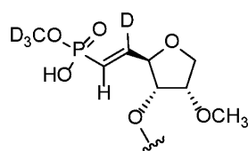
Formula (12BY)
