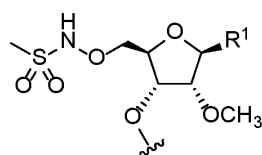
Formula (14)
