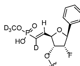
Formula (31AY)
