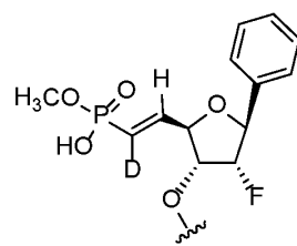
Formula (31AX)
