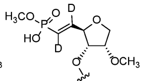
Formula (10BX)
