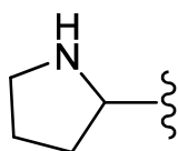
pyrrolidin-2-yl “heterocyclyl group”
