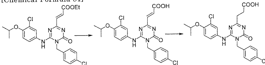
[Chemical Formula 81]
