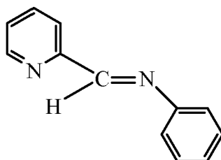
Imine C
