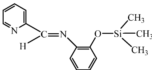
Imine A
