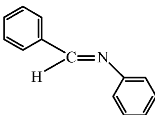
Imine B
