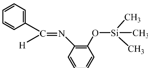
Imine D
