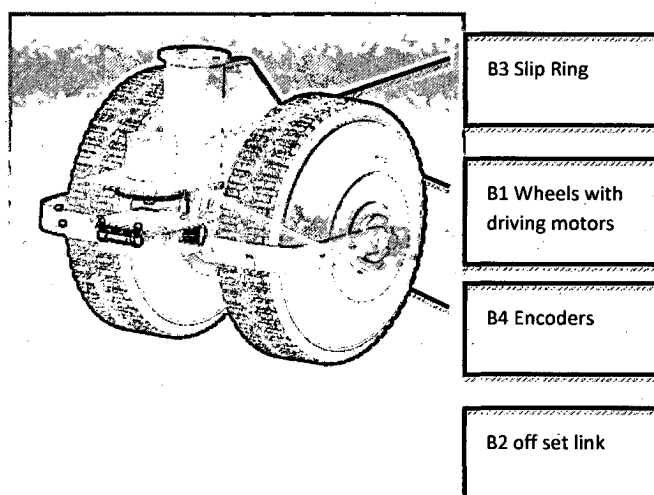
Figure 3. Omni-directional module
