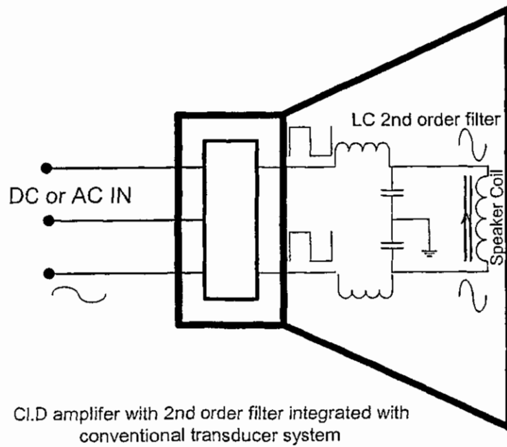
Figure 2 (prior art)
