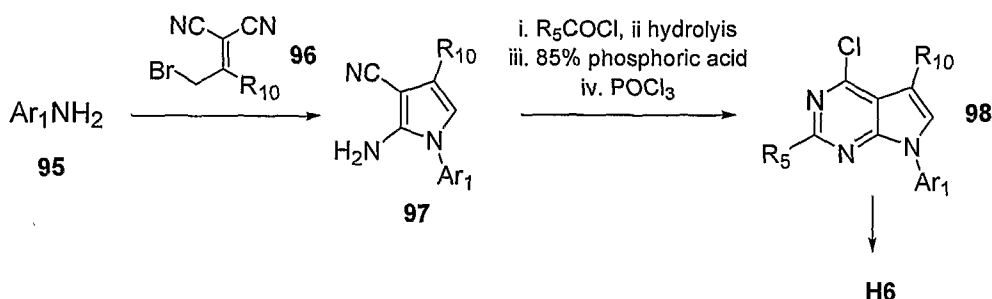
Scheme 19a
