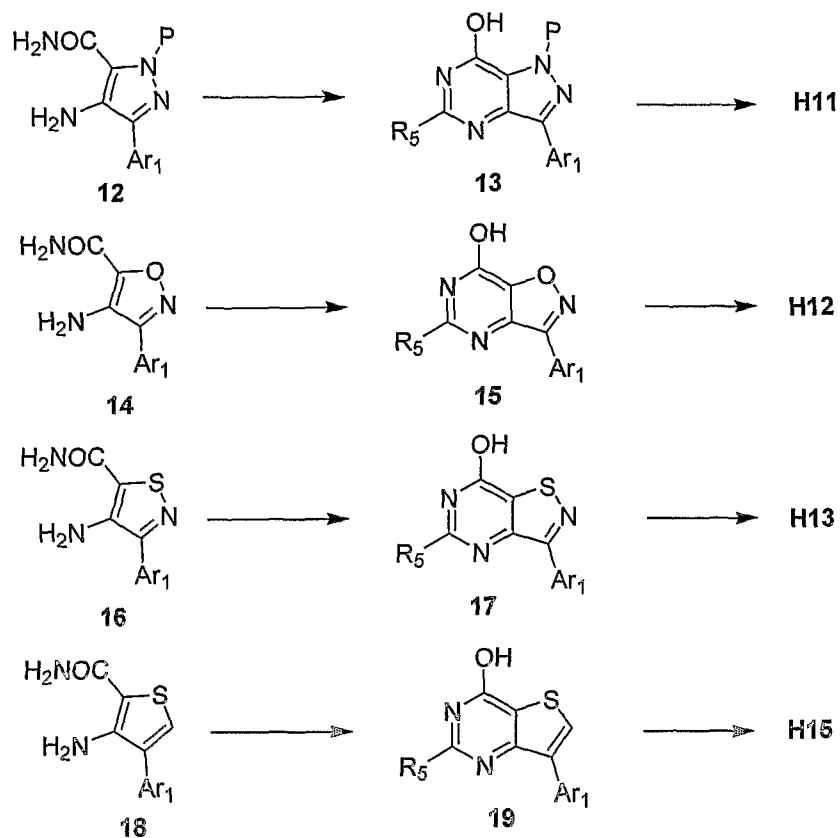
Scheme 4
