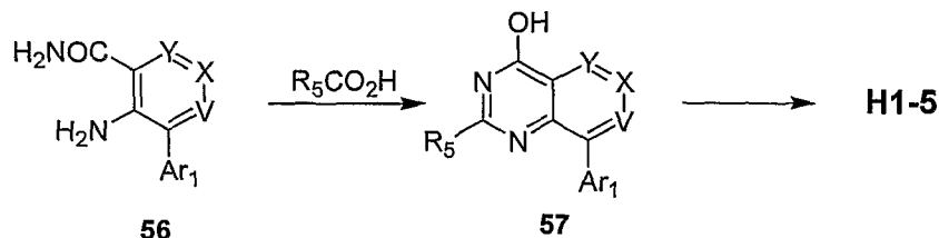
Scheme 12
