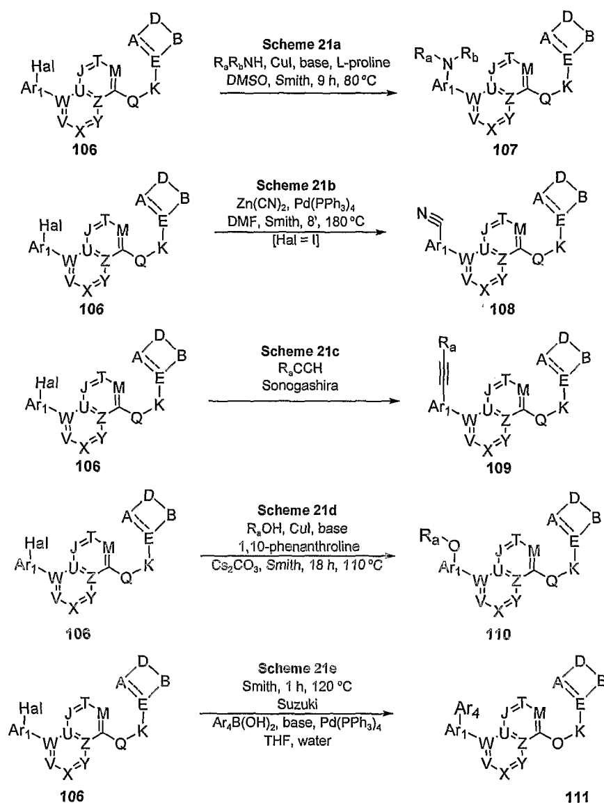
Scheme 21
