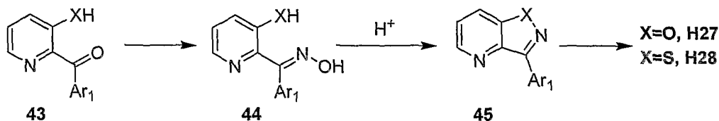
Scheme 9
