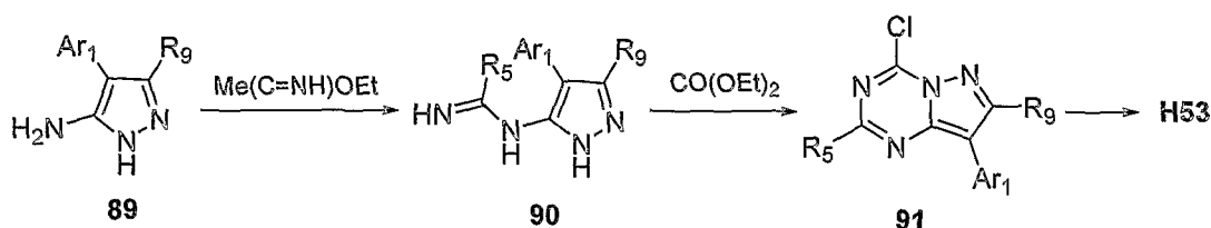
Scheme 18b
