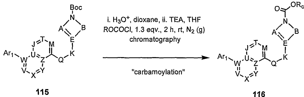
Scheme 23
