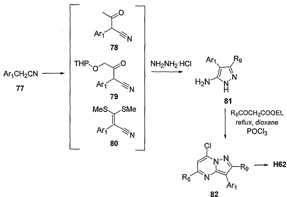
Scheme 17
