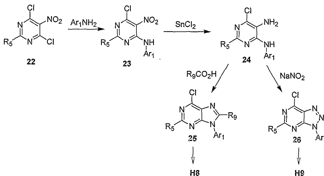
Scheme 5
