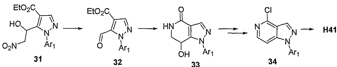
Scheme 6b
