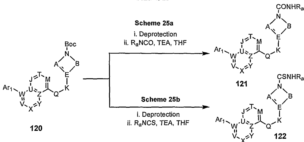
Scheme 25
