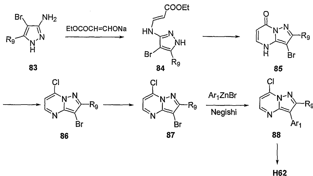
Scheme 18
