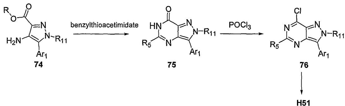
149 Scheme 16
