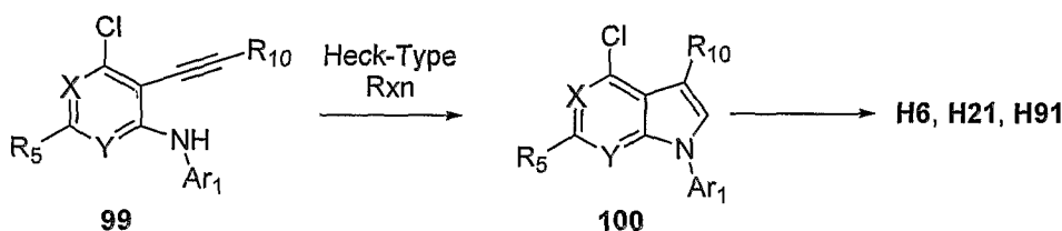
Scheme 19b
