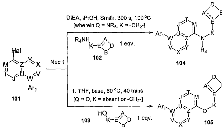
Scheme 20
