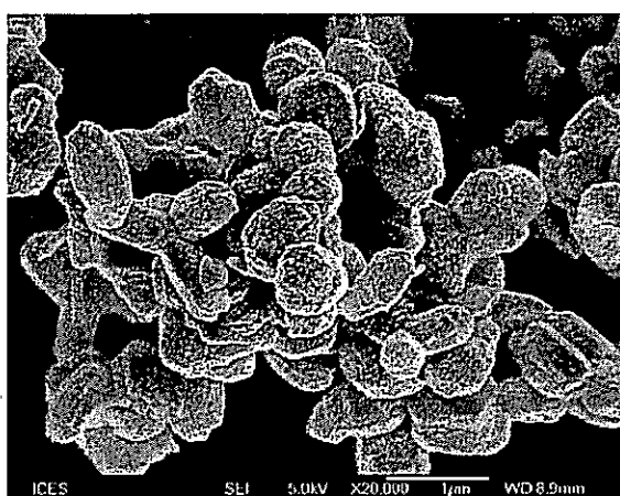
Mesoporous Carbon
