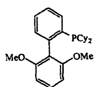
S Phos
