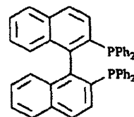
Rac-BINAP
