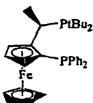
FC_B
