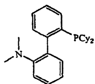
Cycloph_B
