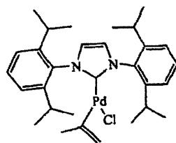
Carbene
