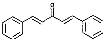
dba (dibenzylideneacetone)
