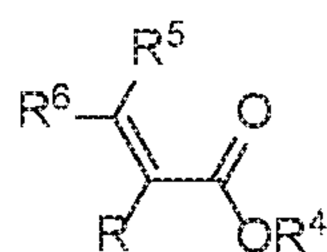
Formula II
