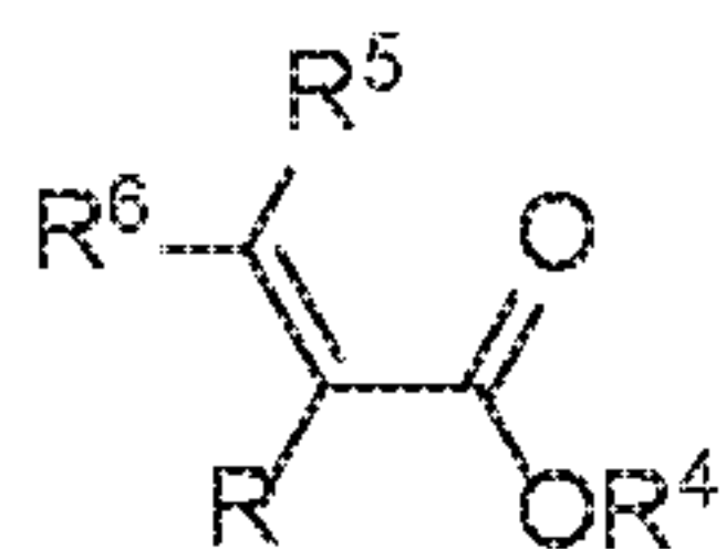
Formula II
