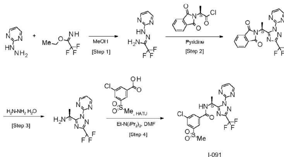
Scheme 15
