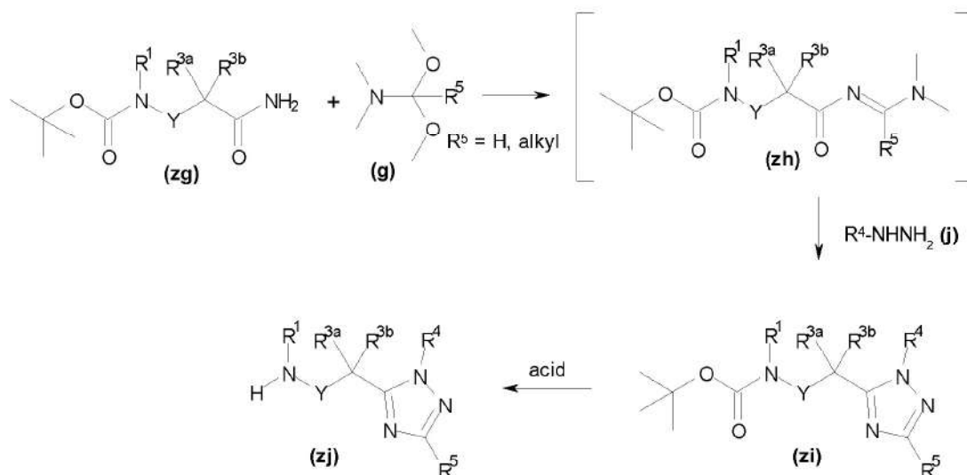
Scheme 11
