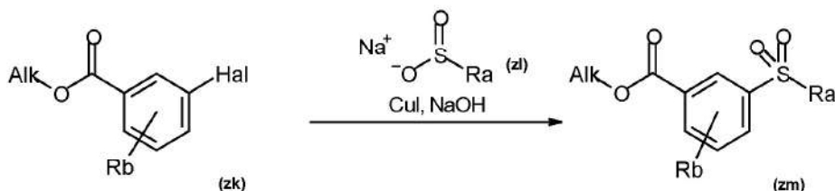
Scheme 12
