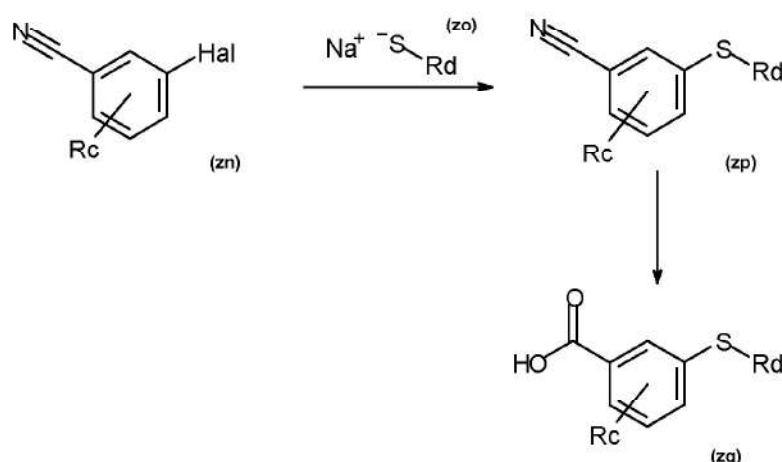
Scheme 13
