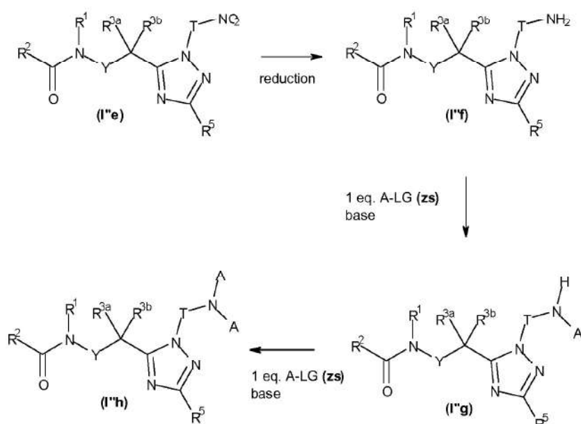
Scheme 16
