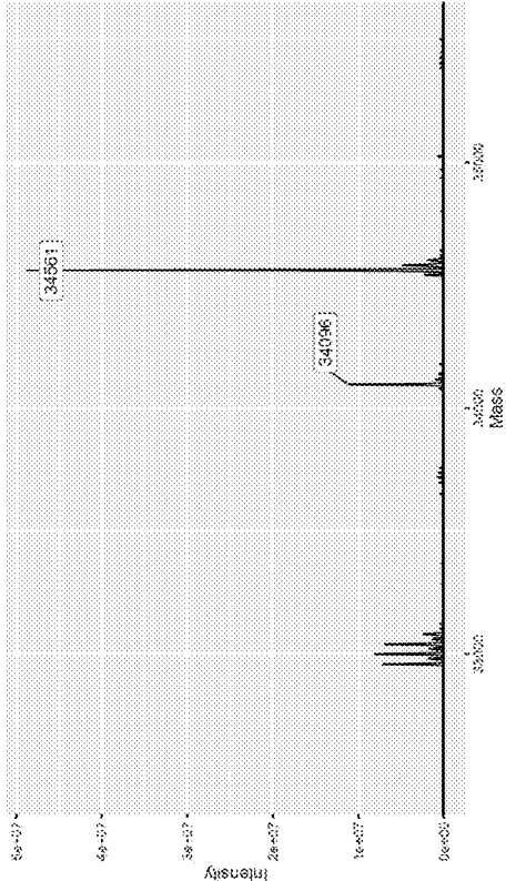
CDK2 + Compound 16
