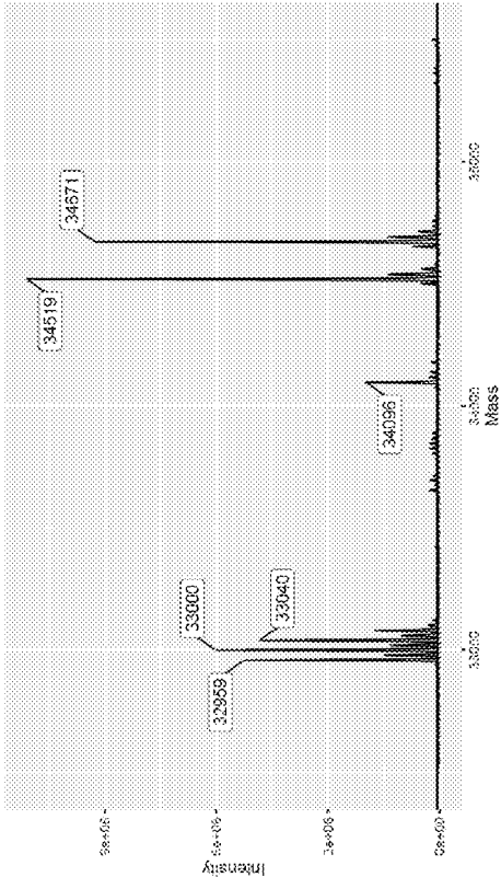
CDK2 + Compound 51
