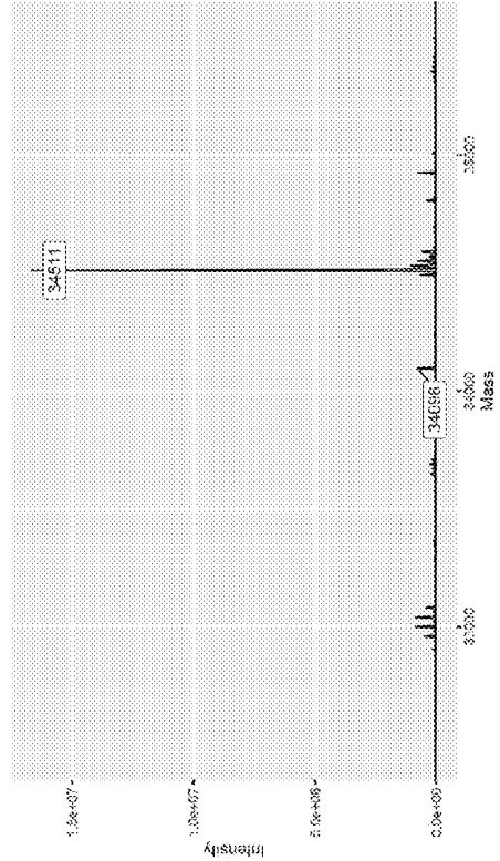
CDK2 + Compound 11
