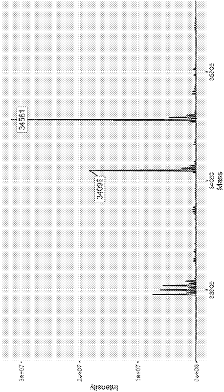
CDK2 + Compound 17
