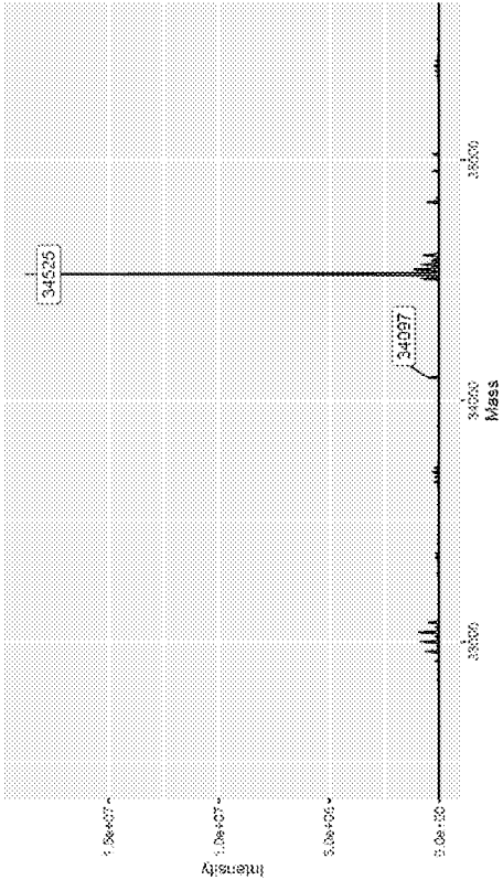
CDK2 + Compound 32
