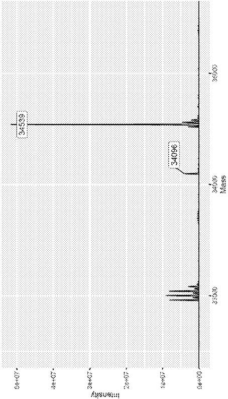
CDK2 + Compound 22
