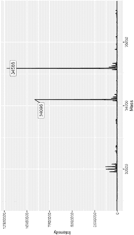
CDK2 + Compound 49
