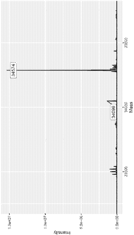
CDK2 + Compound 69
