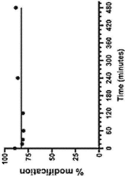
CDK2 + Compound 89
