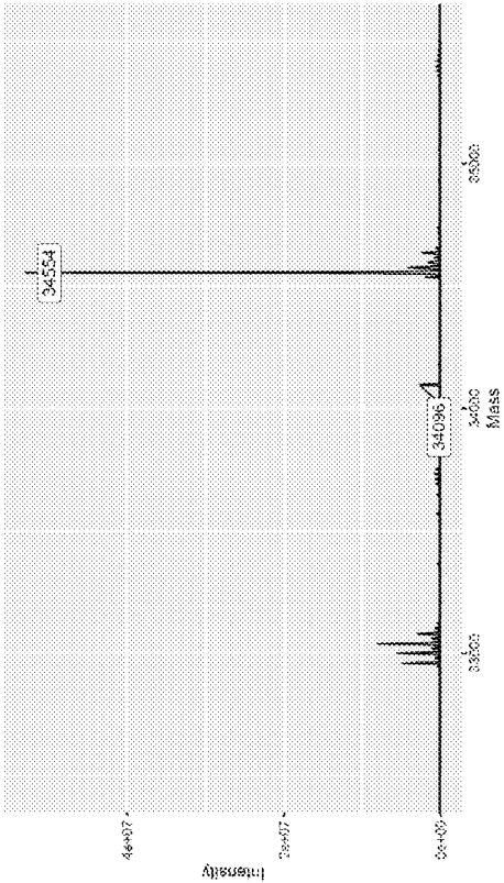
CDK2 + Compound 103
