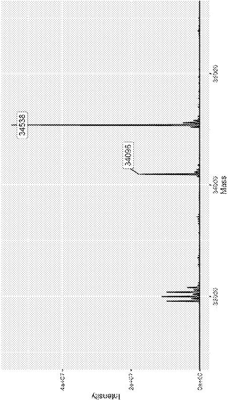
CDK2 + Compound 22
