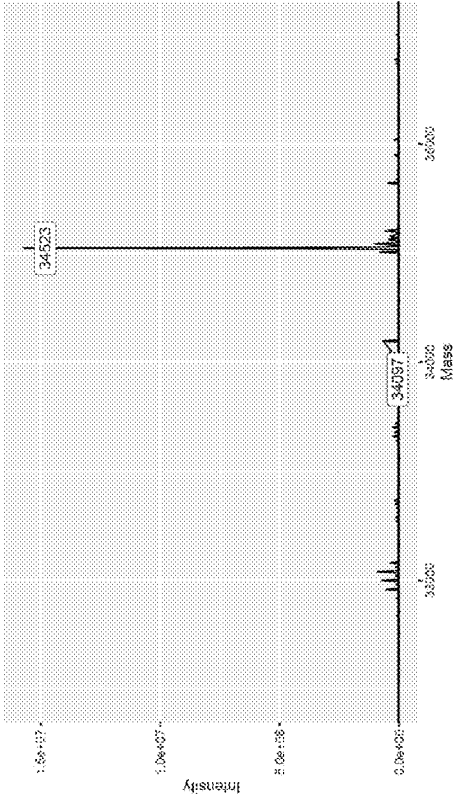
CDK2 + Compound 82
