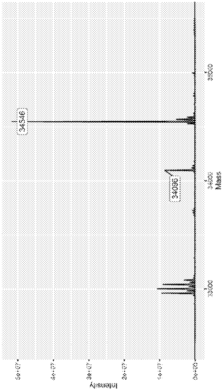
CDK2 + Compound 13
