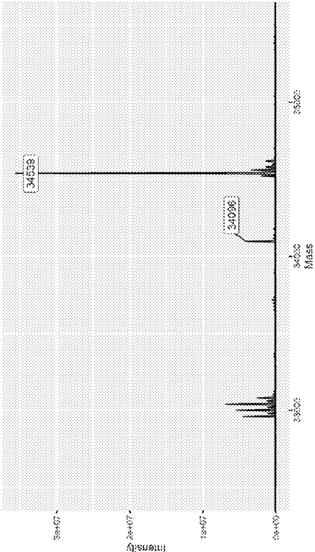
CDK2 + Compound 64
