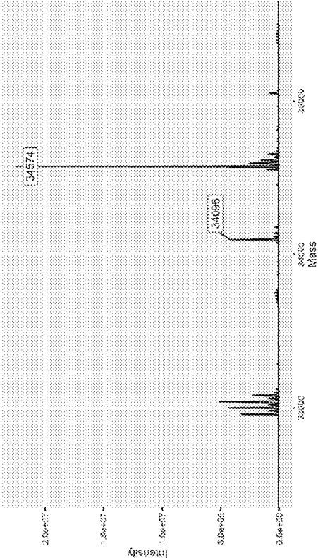
CDK2 + Compound 69
