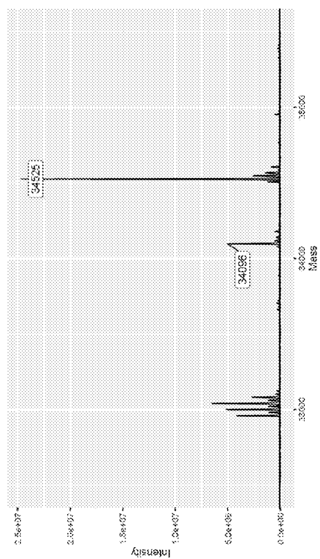
CDK2 + Compound 32
