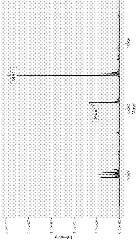
CDK2 + Compound 11
