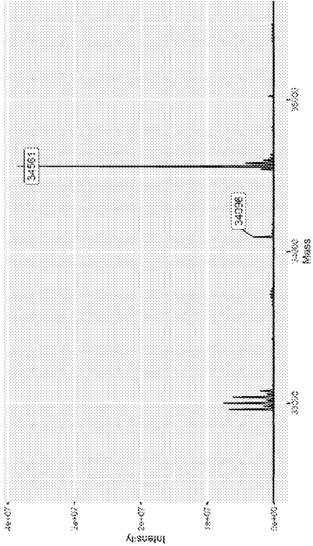
CDK2 + Compound 17
