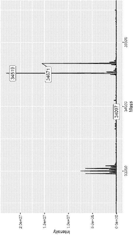
CDK2 + Compound 51
