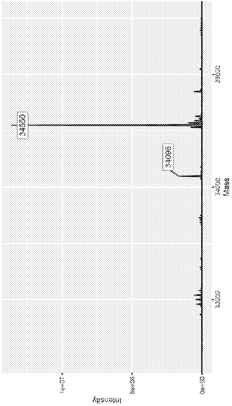
CDK2 + Compound 89
