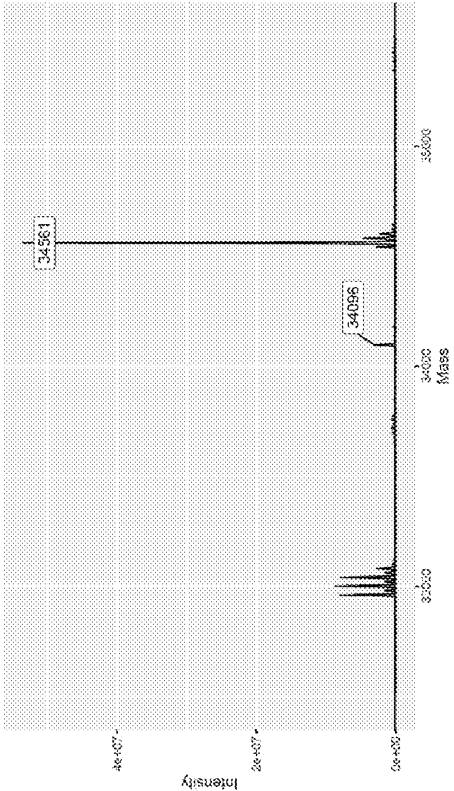
CDK2 + Compound 16
