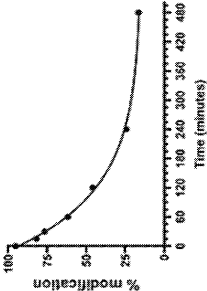
CDK2 + Compound 103
