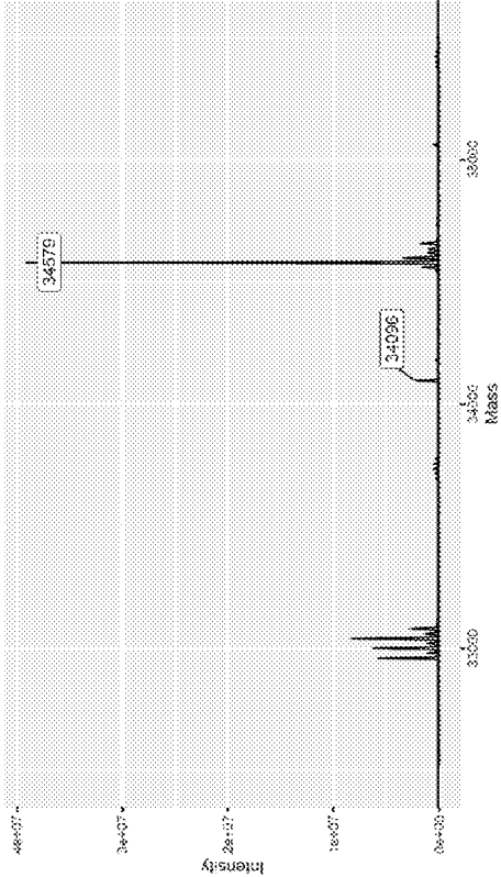
CDK2 + Compound 45
