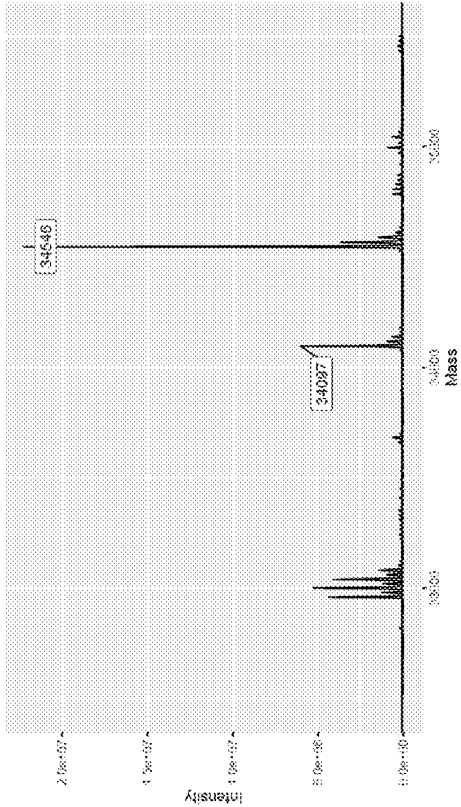
CDK2 + Compound 13
