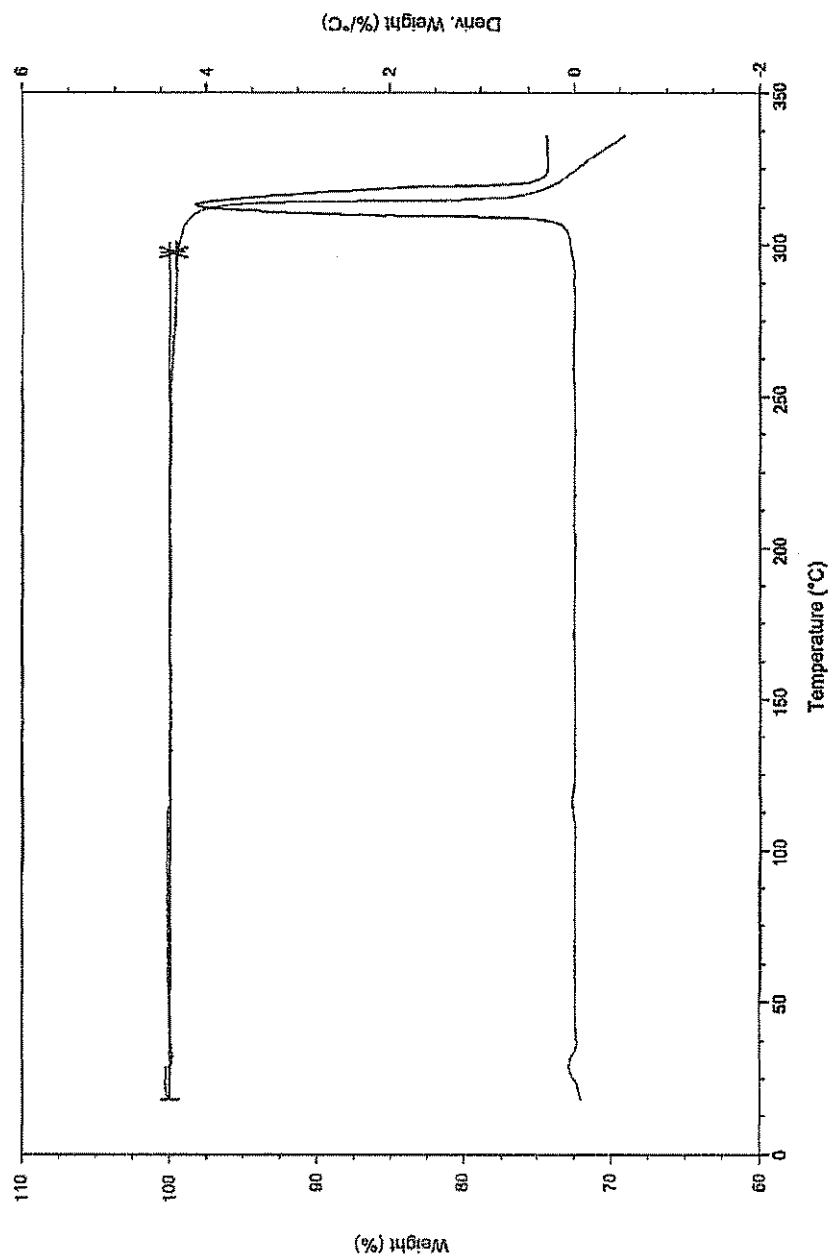
Figure 12 TGA
