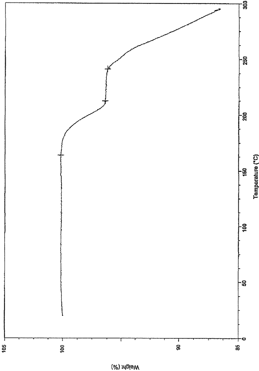
Figure 18 TGA
