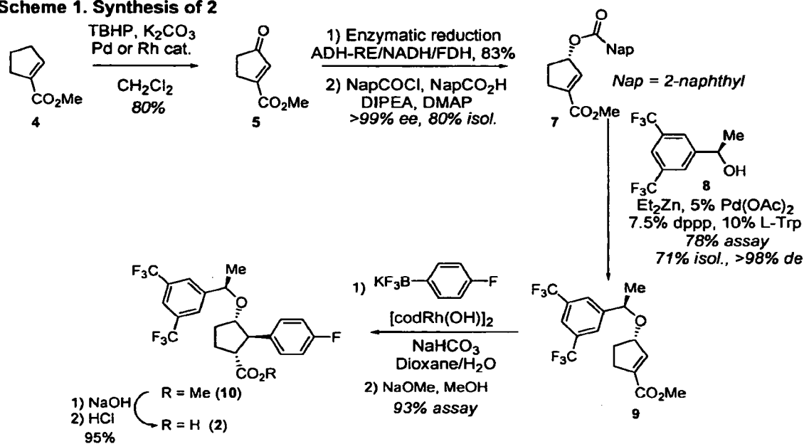
Scheme 1. Synthesis of 2
