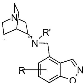
(IIIq)
